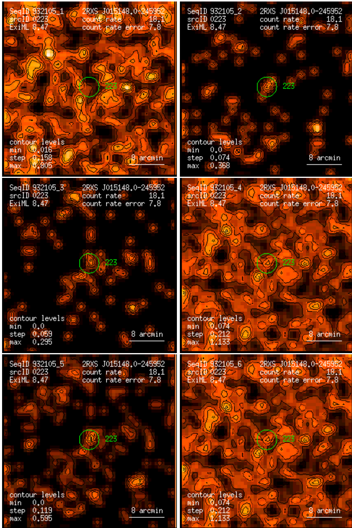
Figure 223: RASS 932105: detection 0223: band rate images, Gaussian filter: (1) PSPC channels 11 – 41, (2) 52 – 90, (3) 91 – 201, (4) 11 – 235, (5) 52 – 201, (6) 11 – 201. Broad band rates in counts/ks. Band rate contour levels in counts/ks/arcmin 2 .
