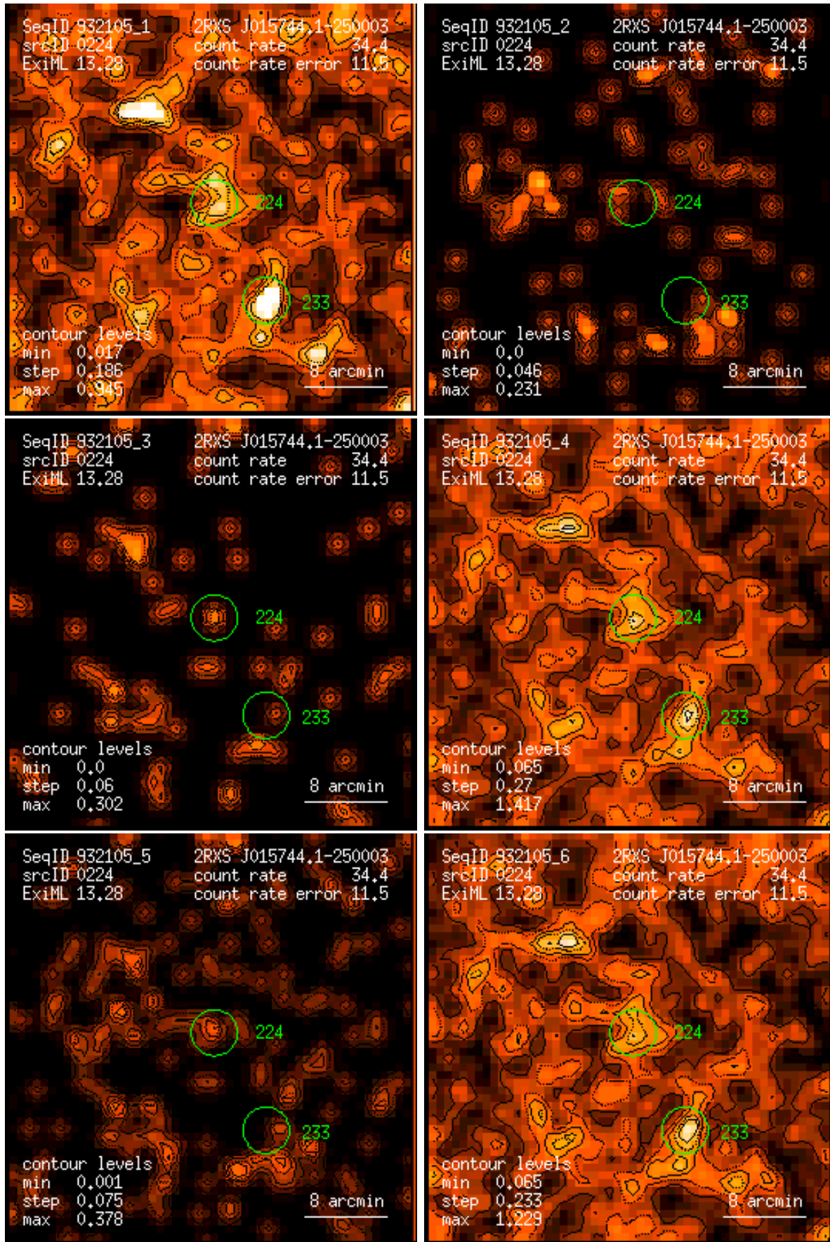
Figure 224: RASS 932105: detection 0224: band rate images, Gaussian filter: (1) PSPC channels 11 – 41, (2) 52 – 90, (3) 91 – 201, (4) 11 – 235, (5) 52 – 201, (6) 11 – 201. Broad band rates in counts/ks. Band rate contour levels in counts/ks/arcmin 2 .
