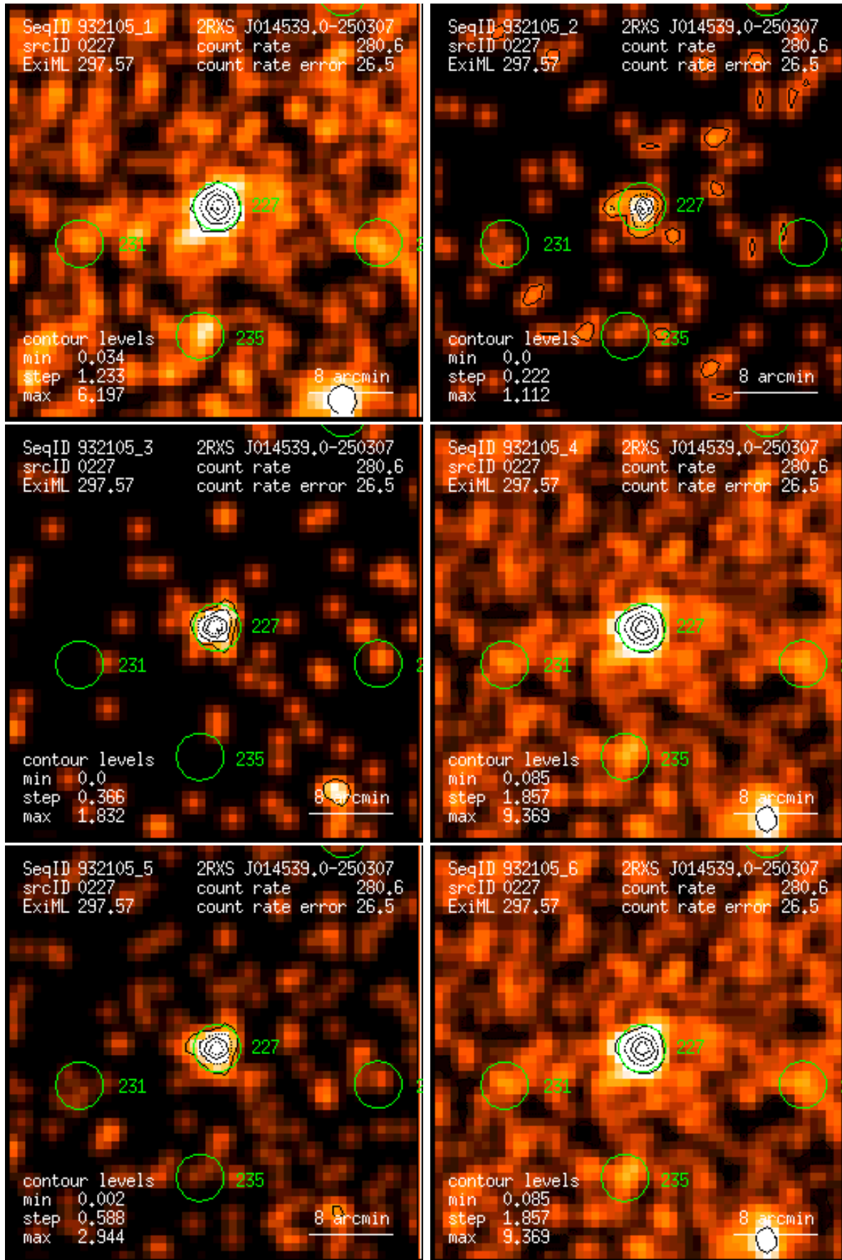
Figure 227: RASS 932105: detection 0227: band rate images, Gaussian filter: (1) PSPC channels 11 – 41, (2) 52 – 90, (3) 91 – 201, (4) 11 – 235, (5) 52 – 201, (6) 11 – 201. Broad band rates in counts/ks. Band rate contour levels in counts/ks/arcmin 2 .
