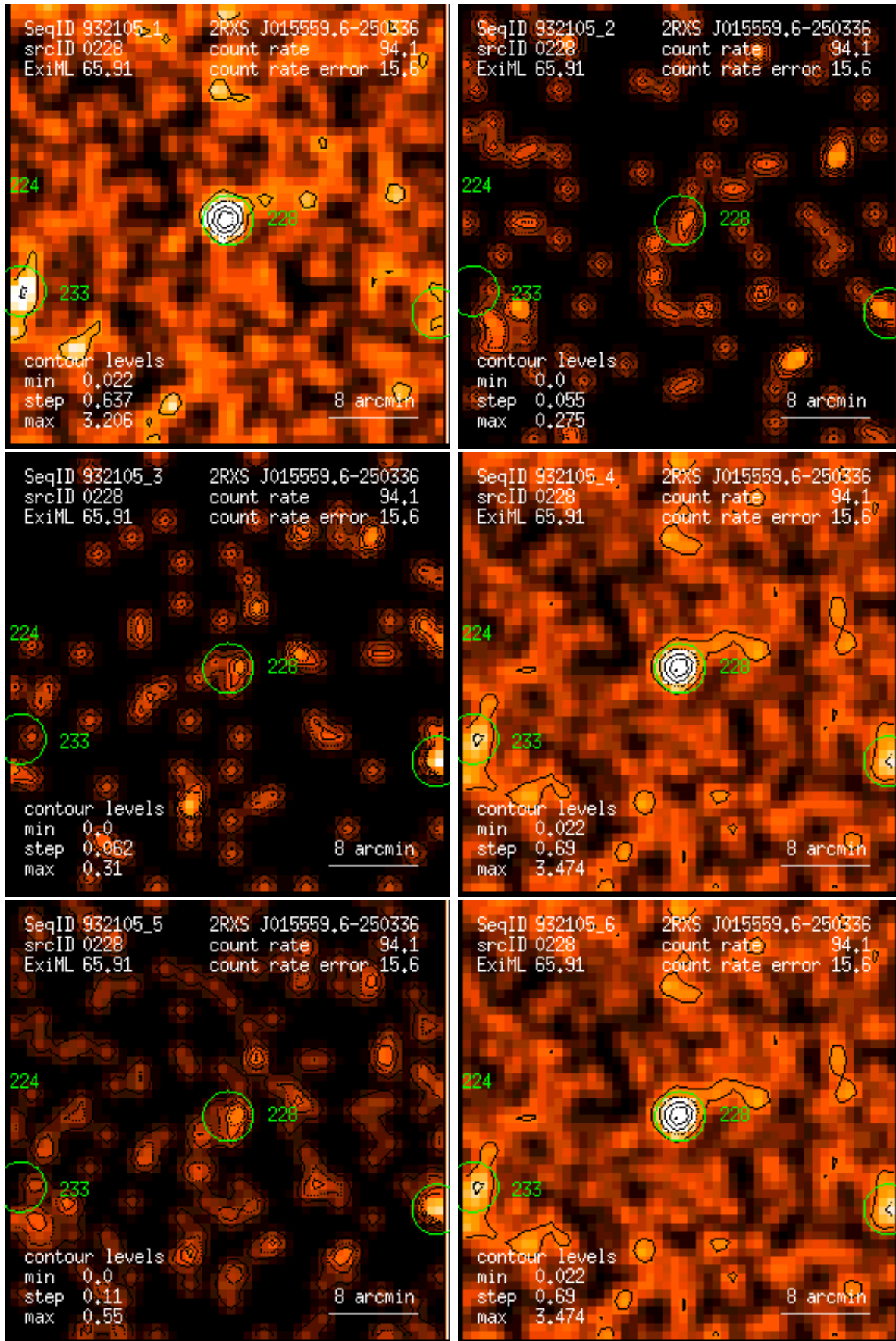
Figure 228: RASS 932105: detection 0228: band rate images, Gaussian filter: (1) PSPC channels 11 – 41, (2) 52 – 90, (3) 91 – 201, (4) 11 – 235, (5) 52 – 201, (6) 11 – 201. Broad band rates in counts/ks. Band rate contour levels in counts/ks/arcmin 2 .
