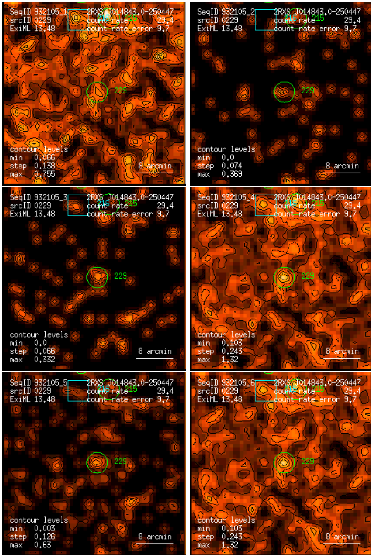
Figure 229: RASS 932105: detection 0229: band rate images, Gaussian filter: (1) PSPC channels 11 – 41, (2) 52 – 90, (3) 91 – 201, (4) 11 – 235, (5) 52 – 201, (6) 11 – 201. Broad band rates in counts/ks. Band rate contour levels in counts/ks/arcmin 2 .
