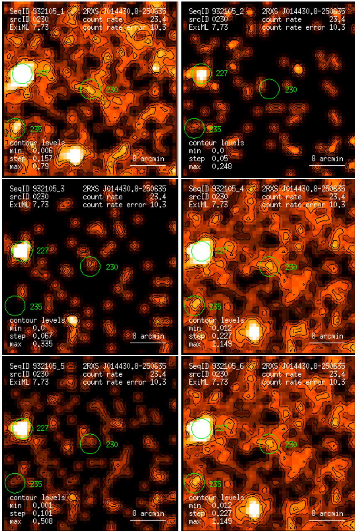
Figure 230: RASS 932105: detection 0230: band rate images, Gaussian filter: (1) PSPC channels 11 – 41, (2) 52 – 90, (3) 91 – 201, (4) 11 – 235, (5) 52 – 201, (6) 11 – 201. Broad band rates in counts/ks. Band rate contour levels in counts/ks/arcmin 2 .
