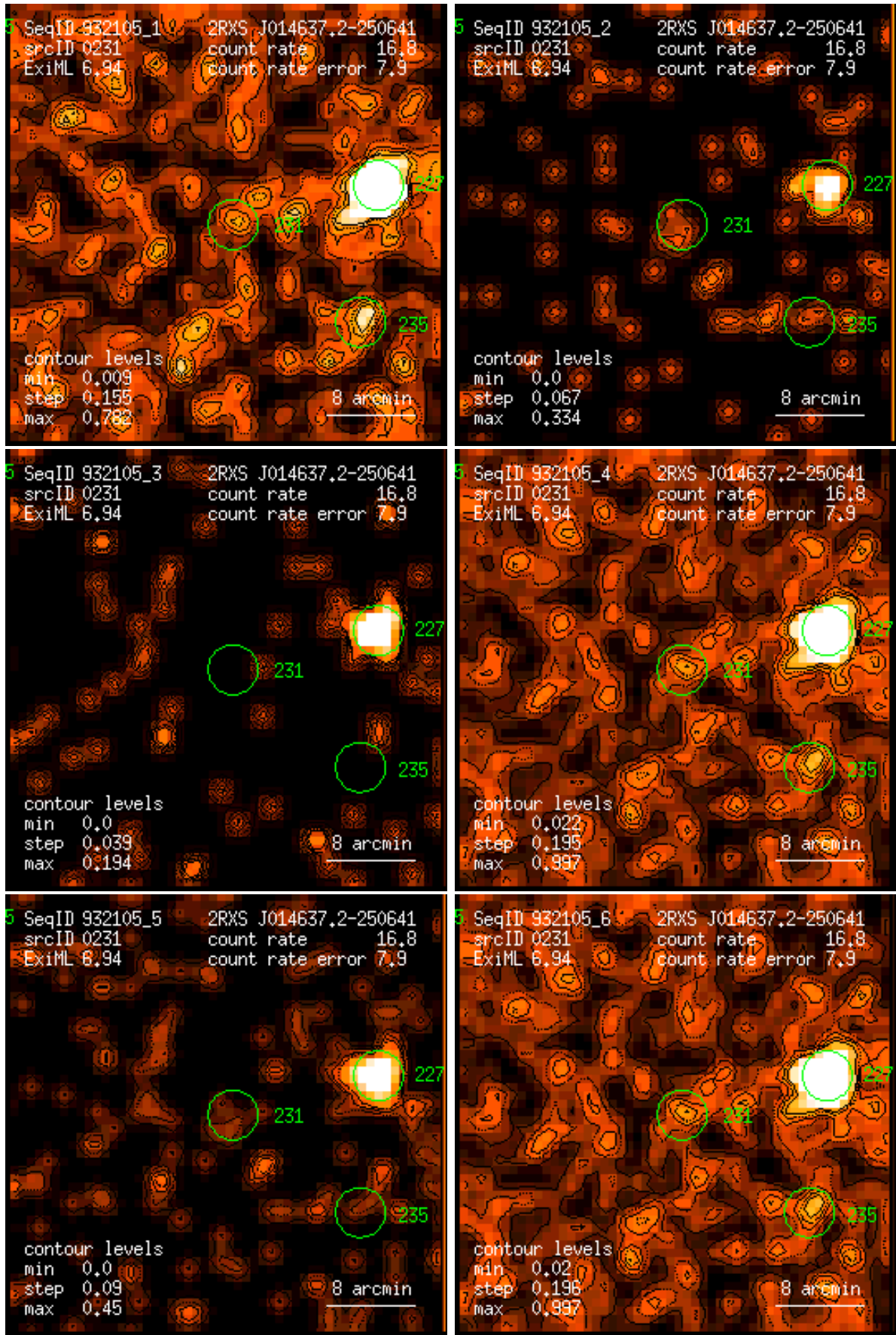
Figure 231: RASS 932105: detection 0231: band rate images, Gaussian filter: (1) PSPC channels 11 – 41, (2) 52 – 90, (3) 91 – 201, (4) 11 – 235, (5) 52 – 201, (6) 11 – 201. Broad band rates in counts/ks. Band rate contour levels in counts/ks/arcmin 2 .
