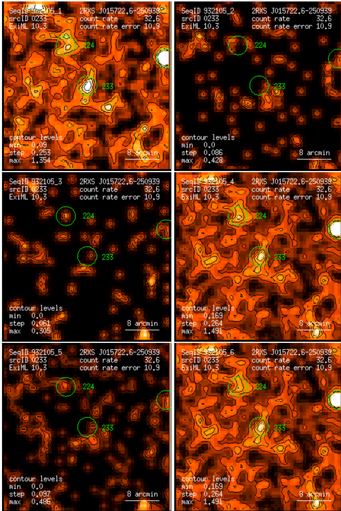
Figure 233: RASS 932105: detection 0233: band rate images, Gaussian filter: (1) PSPC channels 11 – 41, (2) 52 – 90, (3) 91 – 201, (4) 11 – 235, (5) 52 – 201, (6) 11 – 201. Broad band rates in counts/ks. Band rate contour levels in counts/ks/arcmin 2 .
