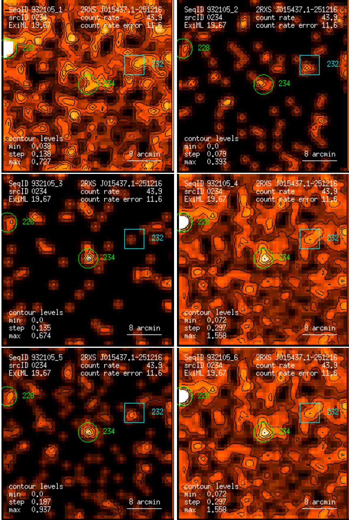
Figure 234: RASS 932105: detection 0234: band rate images, Gaussian filter: (1) PSPC channels 11 – 41, (2) 52 – 90, (3) 91 – 201, (4) 11 – 235, (5) 52 – 201, (6) 11 – 201. Broad band rates in counts/ks. Band rate contour levels in counts/ks/arcmin 2 .
