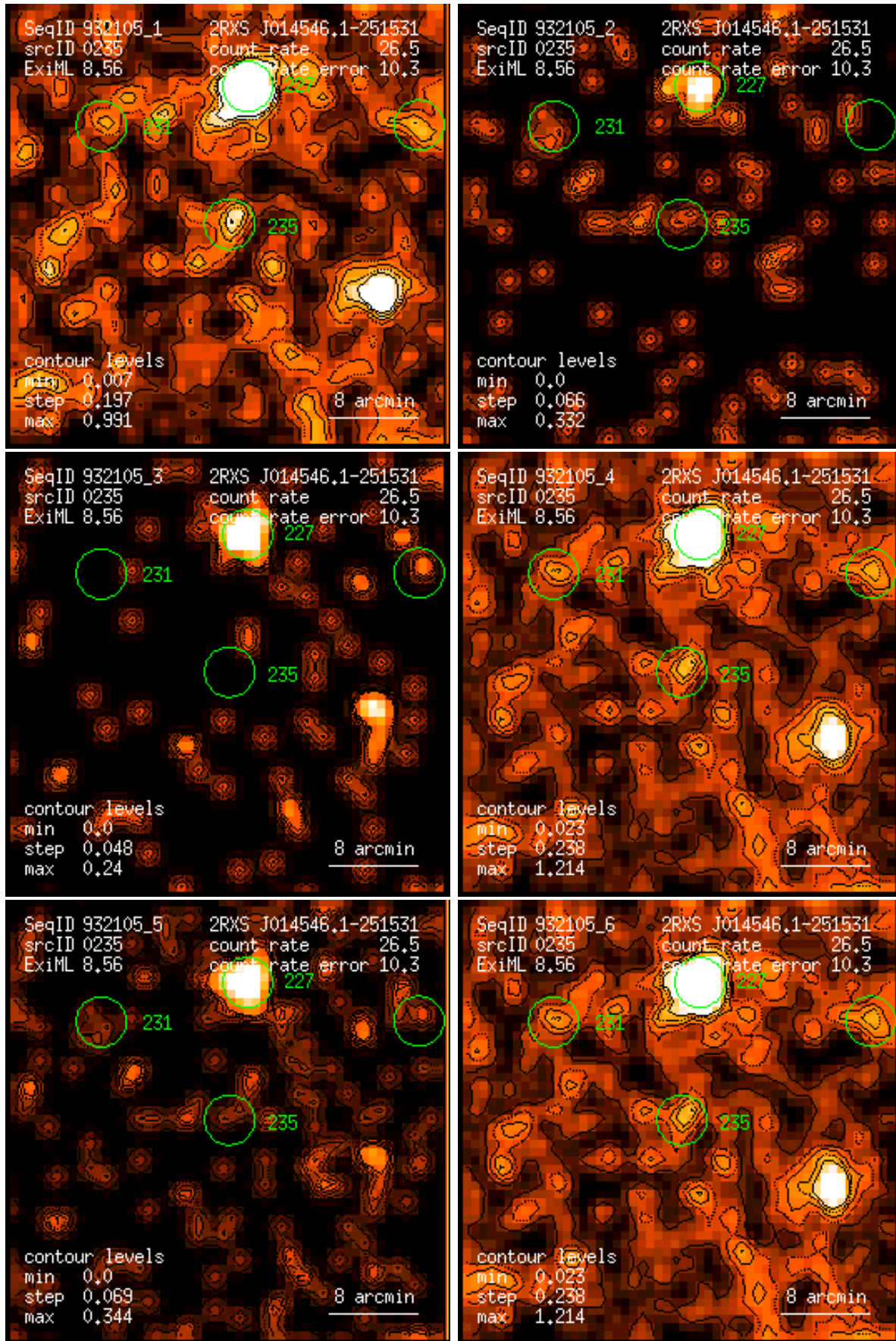
Figure 235: RASS 932105: detection 0235: band rate images, Gaussian filter: (1) PSPC channels 11 – 41, (2) 52 – 90, (3) 91 – 201, (4) 11 – 235, (5) 52 – 201, (6) 11 – 201. Broad band rates in counts/ks. Band rate contour levels in counts/ks/arcmin 2 .
