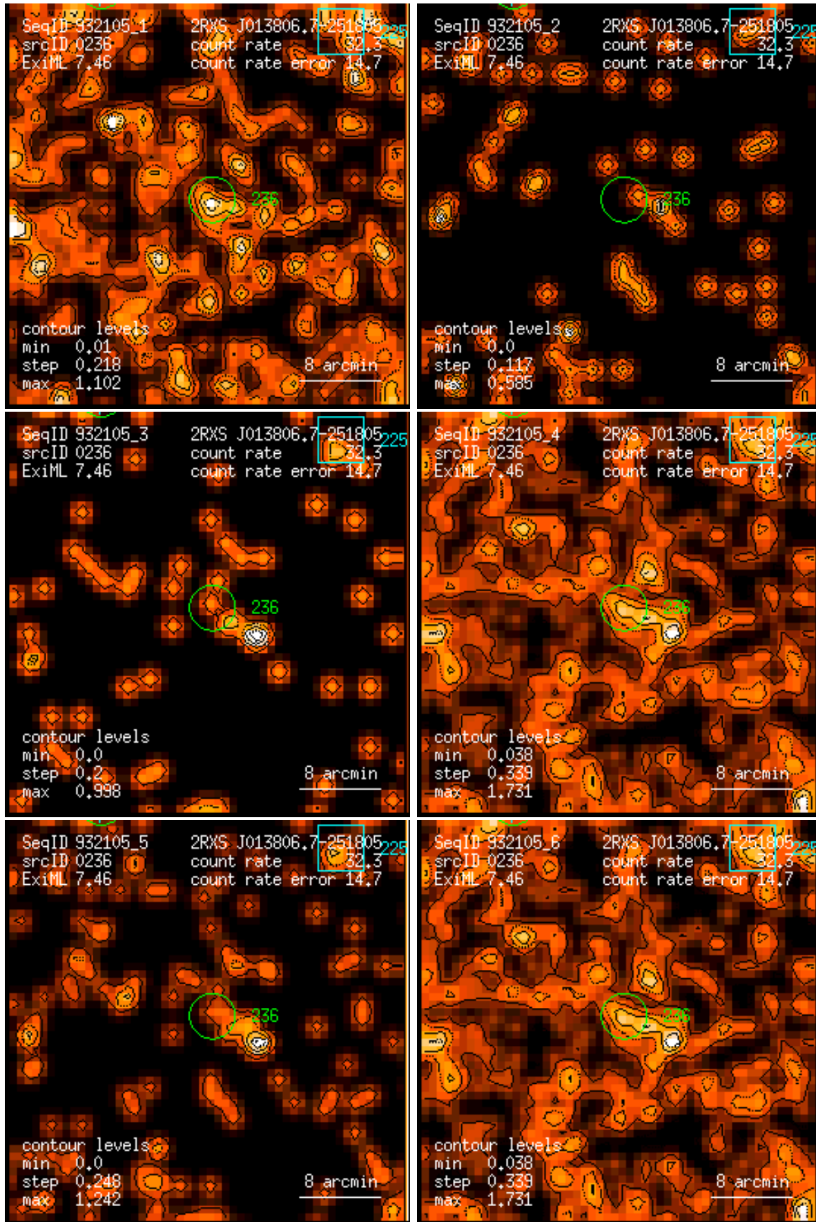
Figure 236: RASS 932105: detection 0236: band rate images, Gaussian filter: (1) PSPC channels 11 – 41, (2) 52 – 90, (3) 91 – 201, (4) 11 – 235, (5) 52 – 201, (6) 11 – 201. Broad band rates in counts/ks. Band rate contour levels in counts/ks/arcmin 2 .
