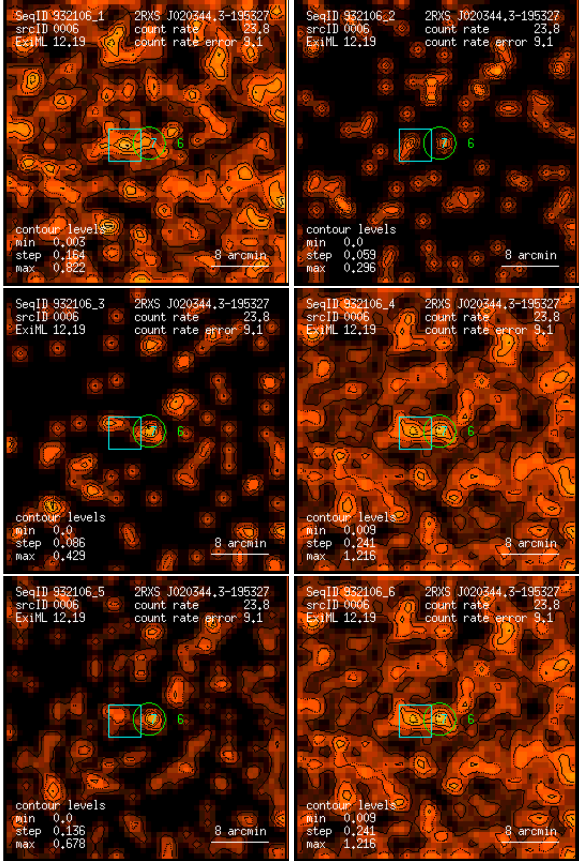
Figure 6: RASS 932106: detection 0006: band rate images, Gaussian filter: (1) PSPC channels 11 – 41, (2) 52 – 90, (3) 91 – 201, (4) 11 – 235, (5) 52 – 201, (6) 11 – 201. Broad band rates in counts/ks. Band rate contour levels in counts/ks/arcmin 2 .
