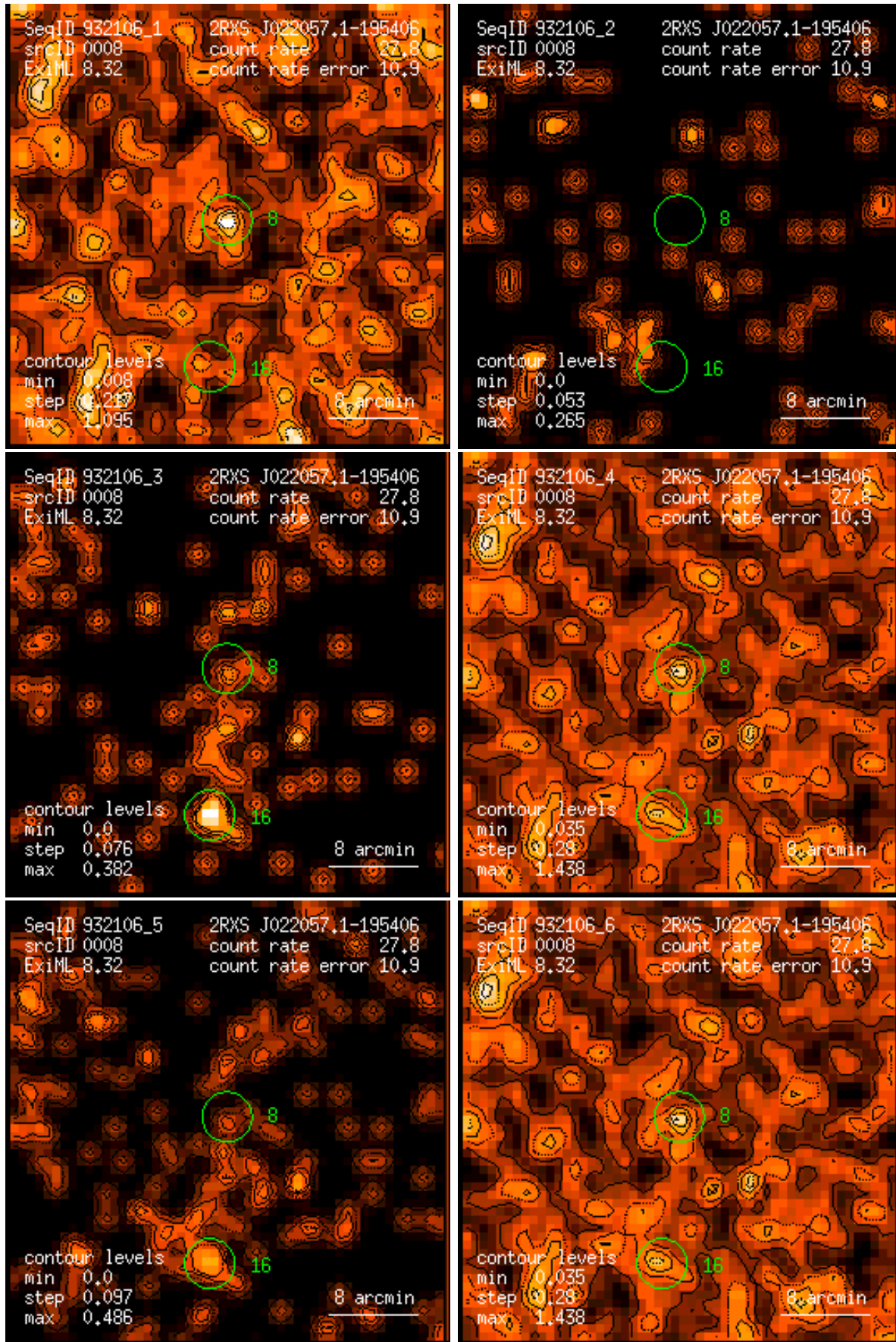
Figure 8: RASS 932106: detection 0008: band rate images, Gaussian filter: (1) PSPC channels 11 – 41, (2) 52 – 90, (3) 91 – 201, (4) 11 – 235, (5) 52 – 201, (6) 11 – 201. Broad band rates in counts/ks. Band rate contour levels in counts/ks/arcmin 2 .
