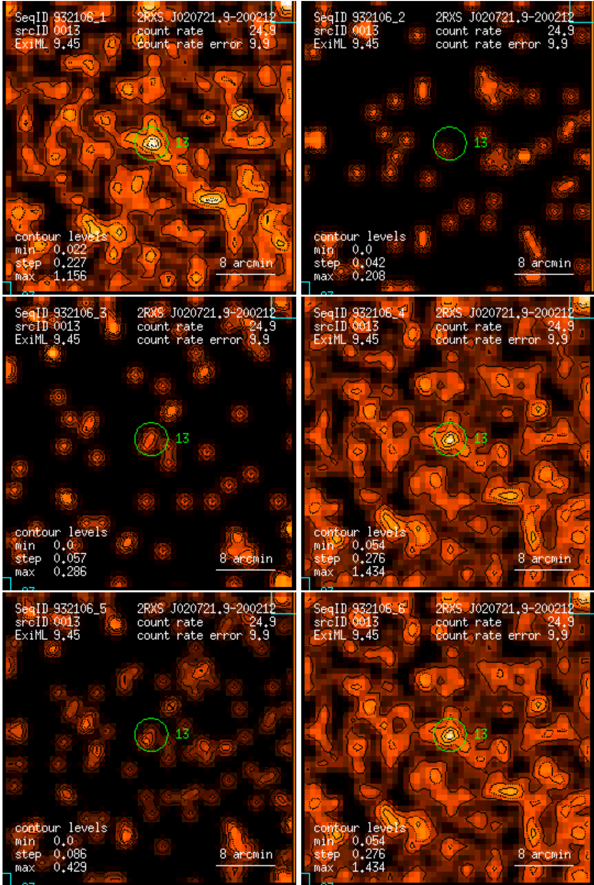
Figure 13: RASS 932106: detection 0013: band rate images, Gaussian filter: (1) PSPC channels 11 – 41, (2) 52 – 90, (3) 91 – 201, (4) 11 – 235, (5) 52 – 201, (6) 11 – 201. Broad band rates in counts/ks. Band rate contour levels in counts/ks/arcmin 2 .
