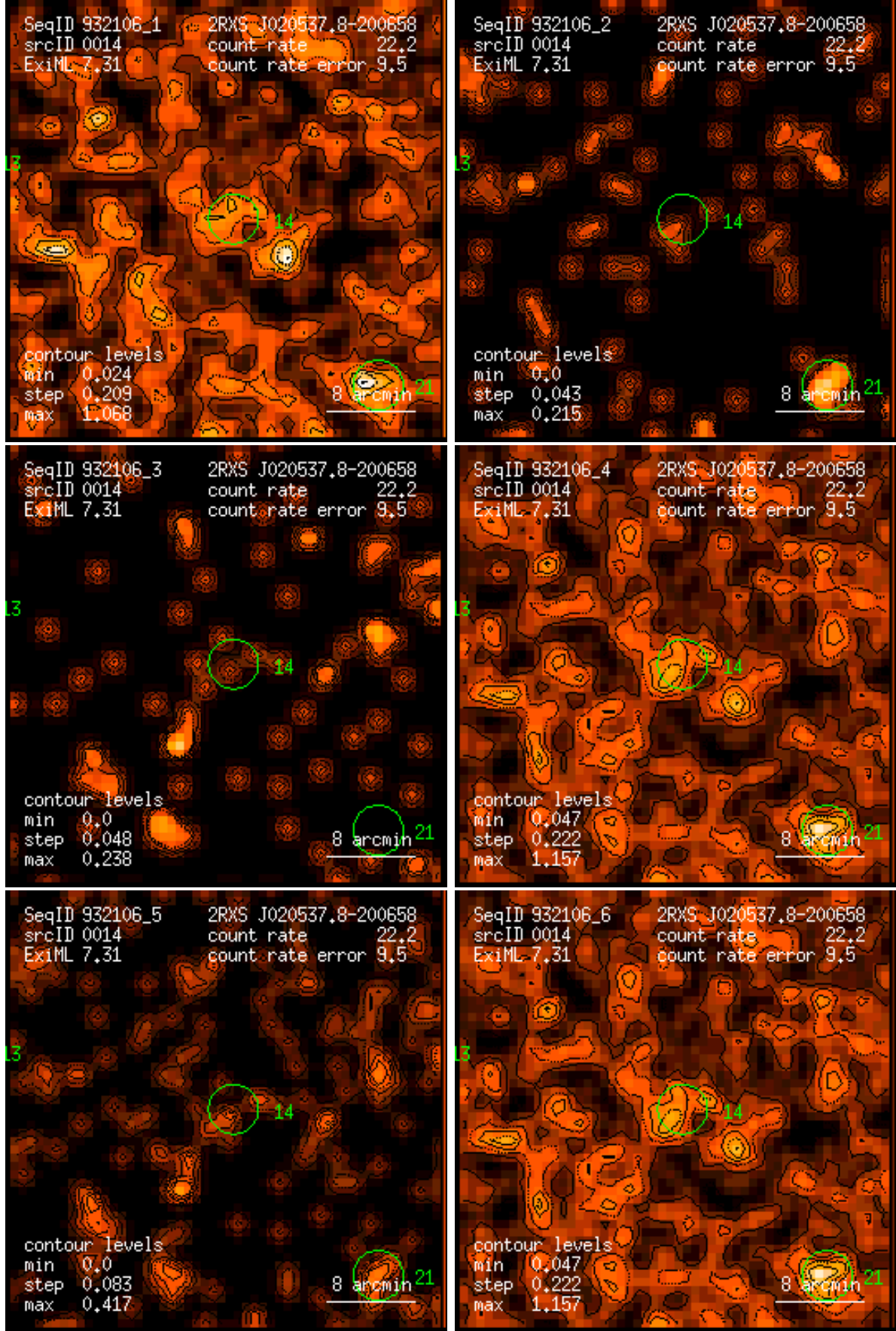
Figure 14: RASS 932106: detection 0014: band rate images, Gaussian filter: (1) PSPC channels 11 – 41, (2) 52 – 90, (3) 91 – 201, (4) 11 – 235, (5) 52 – 201, (6) 11 – 201. Broad band rates in counts/ks. Band rate contour levels in counts/ks/arcmin 2 .
