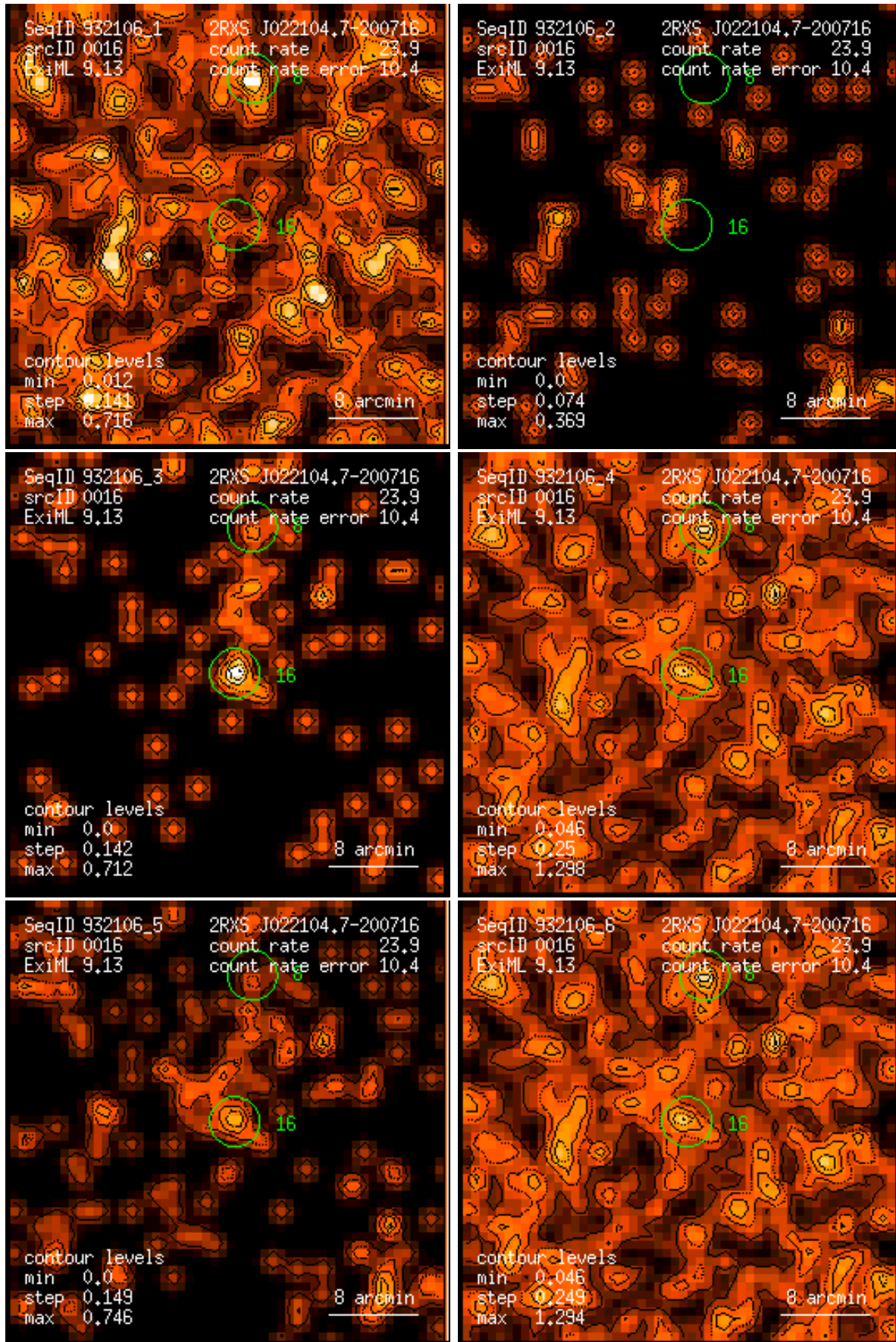
Figure 16: RASS 932106: detection 0016: band rate images, Gaussian filter: (1) PSPC channels 11 – 41, (2) 52 – 90, (3) 91 – 201, (4) 11 – 235, (5) 52 – 201, (6) 11 – 201. Broad band rates in counts/ks. Band rate contour levels in counts/ks/arcmin 2 .
