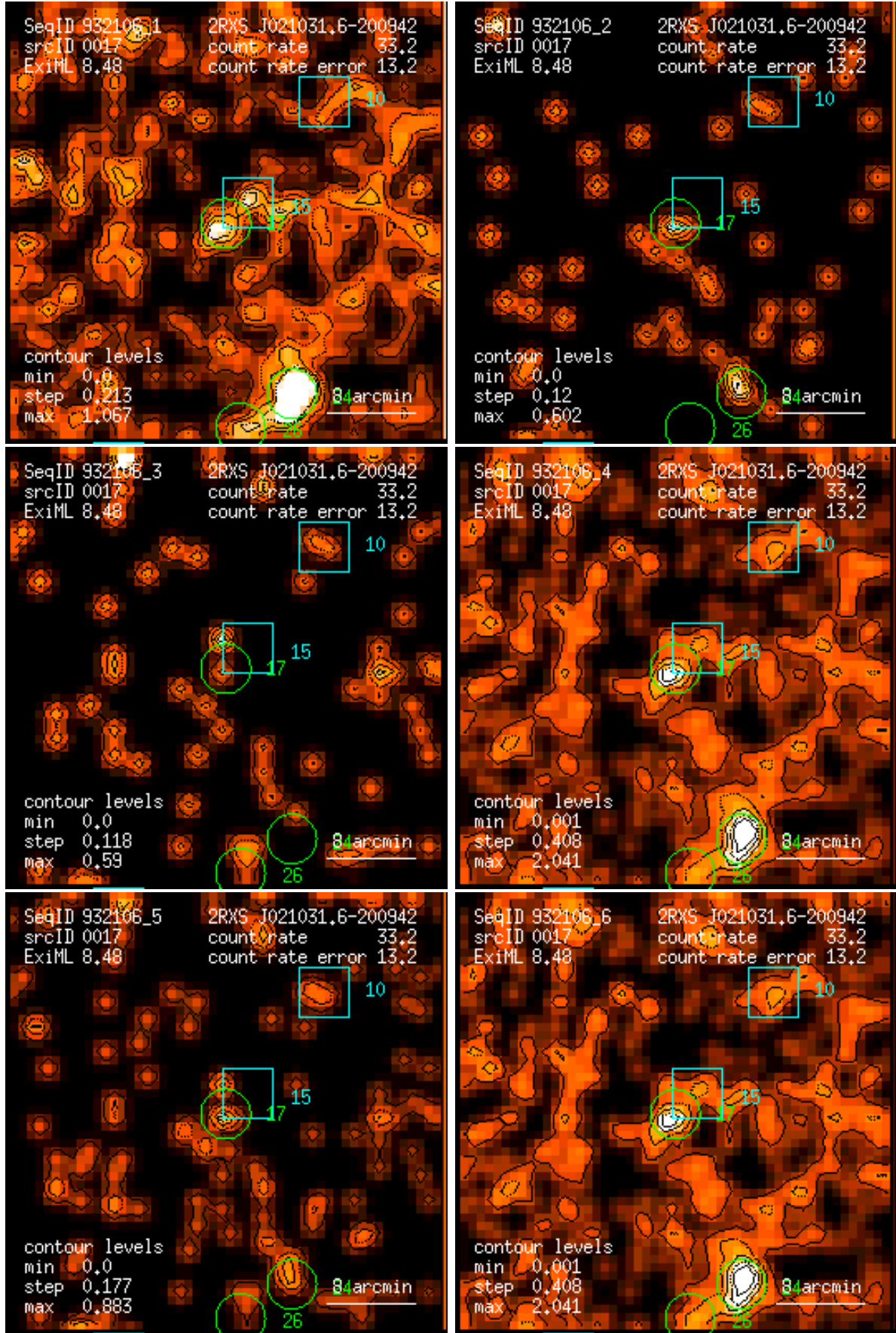
Figure 17: RASS 932106: detection 0017: band rate images, Gaussian filter: (1) PSPC channels 11 – 41, (2) 52 – 90, (3) 91 – 201, (4) 11 – 235, (5) 52 – 201, (6) 11 – 201. Broad band rates in counts/ks. Band rate contour levels in counts/ks/arcmin 2 .
