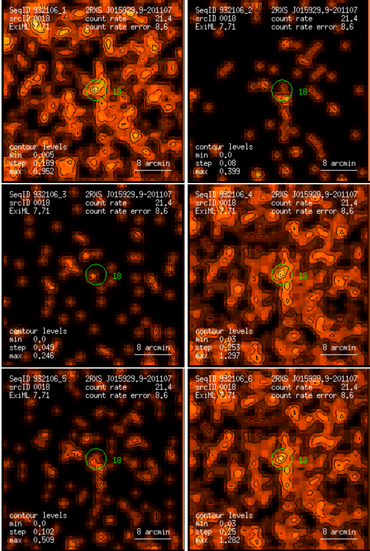
Figure 18: RASS 932106: detection 0018: band rate images, Gaussian filter: (1) PSPC channels 11 – 41, (2) 52 – 90, (3) 91 – 201, (4) 11 – 235, (5) 52 – 201, (6) 11 – 201. Broad band rates in counts/ks. Band rate contour levels in counts/ks/arcmin 2 .
