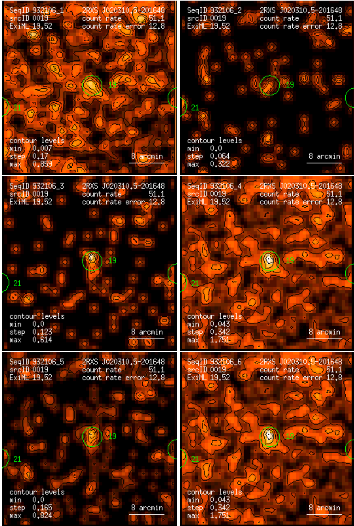
Figure 19: RASS 932106: detection 0019: band rate images, Gaussian filter: (1) PSPC channels 11 – 41, (2) 52 – 90, (3) 91 – 201, (4) 11 – 235, (5) 52 – 201, (6) 11 – 201. Broad band rates in counts/ks. Band rate contour levels in counts/ks/arcmin 2 .
