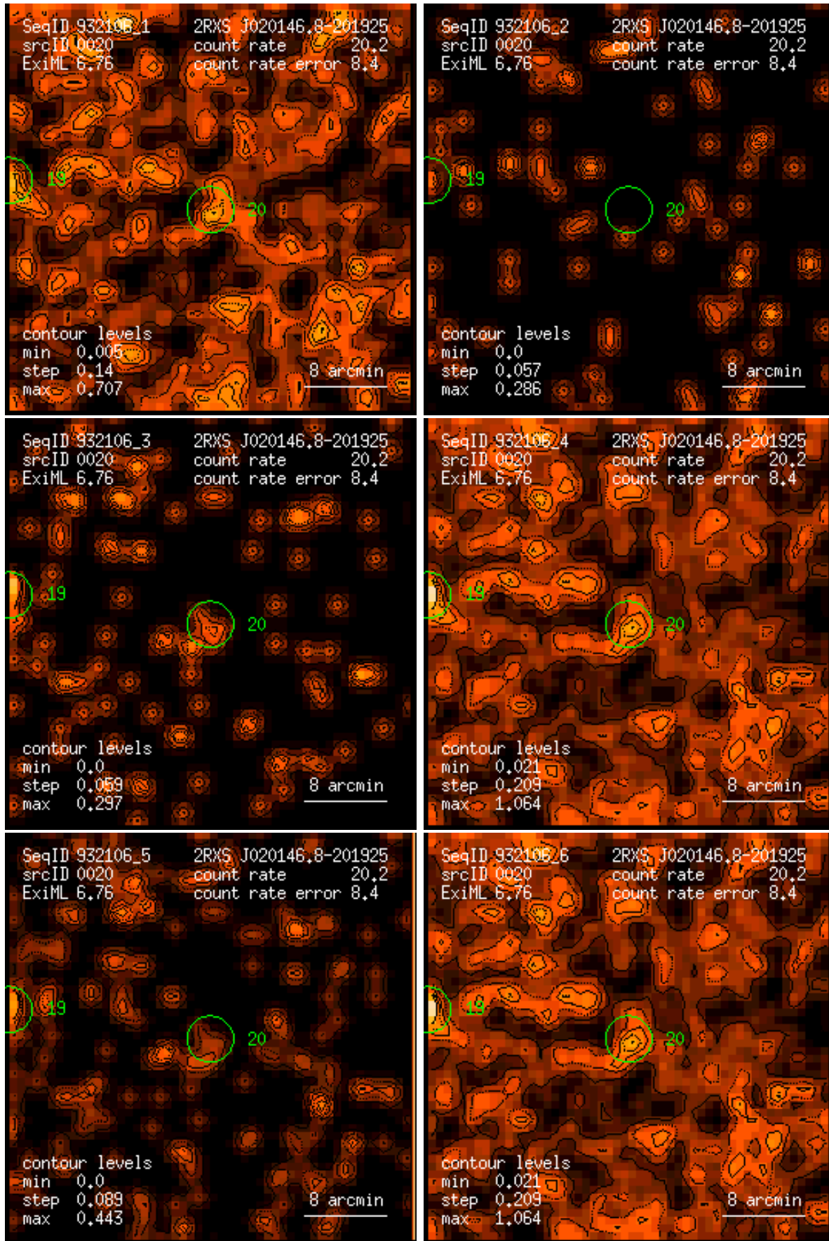
Figure 20: RASS 932106: detection 0020: band rate images, Gaussian filter: (1) PSPC channels 11 – 41, (2) 52 – 90, (3) 91 – 201, (4) 11 – 235, (5) 52 – 201, (6) 11 – 201. Broad band rates in counts/ks. Band rate contour levels in counts/ks/arcmin 2 .
