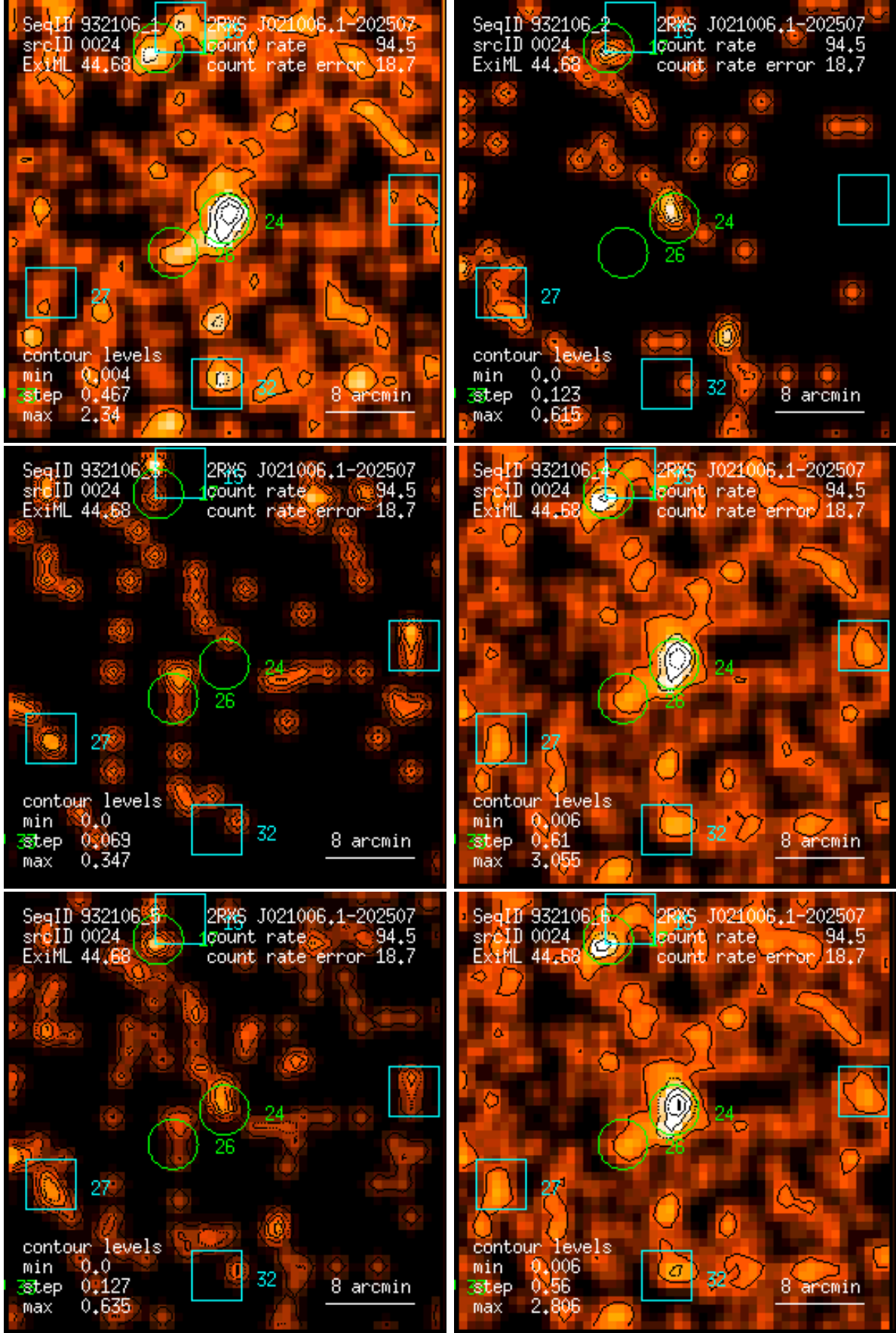
Figure 24: RASS 932106: detection 0024: band rate images, Gaussian filter: (1) PSPC channels 11 – 41, (2) 52 – 90, (3) 91 – 201, (4) 11 – 235, (5) 52 – 201, (6) 11 – 201. Broad band rates in counts/ks. Band rate contour levels in counts/ks/arcmin 2 .
