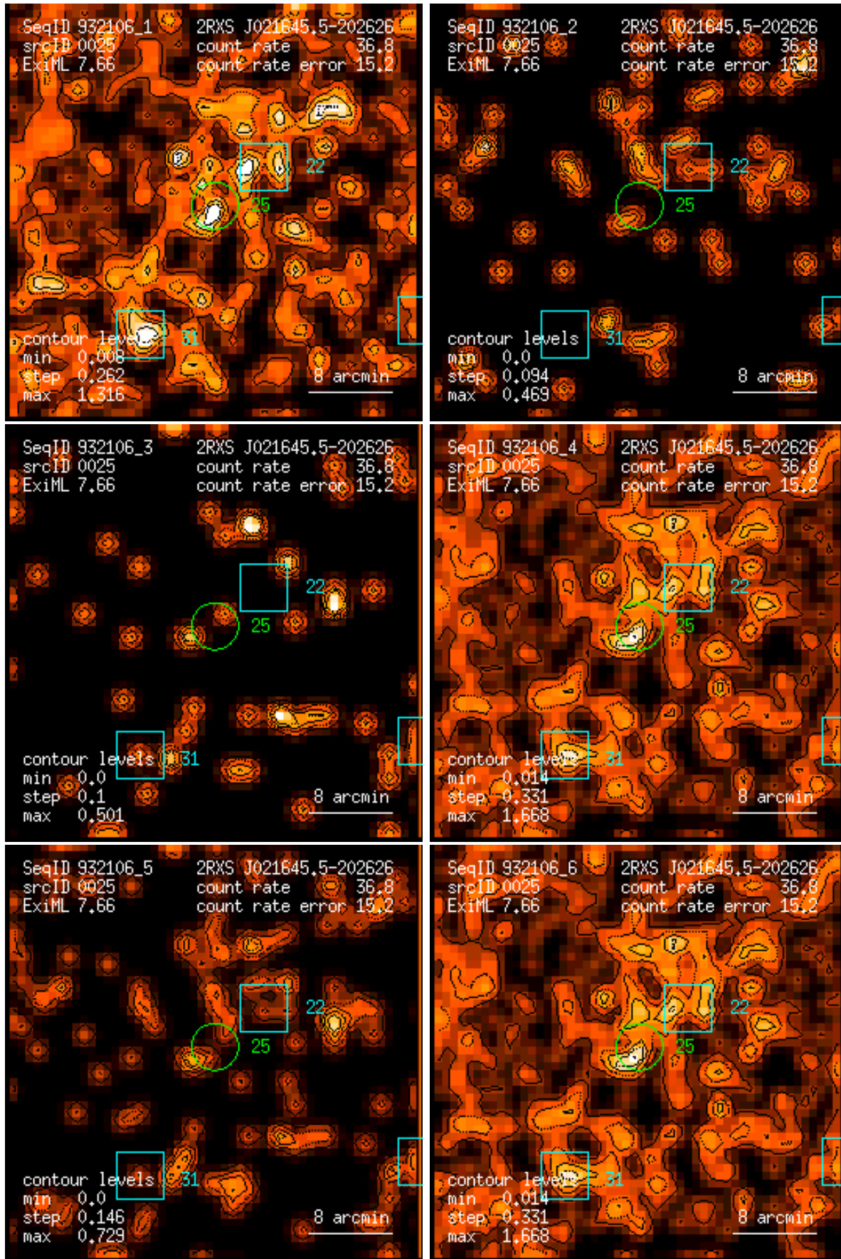
Figure 25: RASS 932106: detection 0025: band rate images, Gaussian filter: (1) PSPC channels 11 – 41, (2) 52 – 90, (3) 91 – 201, (4) 11 – 235, (5) 52 – 201, (6) 11 – 201. Broad band rates in counts/ks. Band rate contour levels in counts/ks/arcmin 2 .
