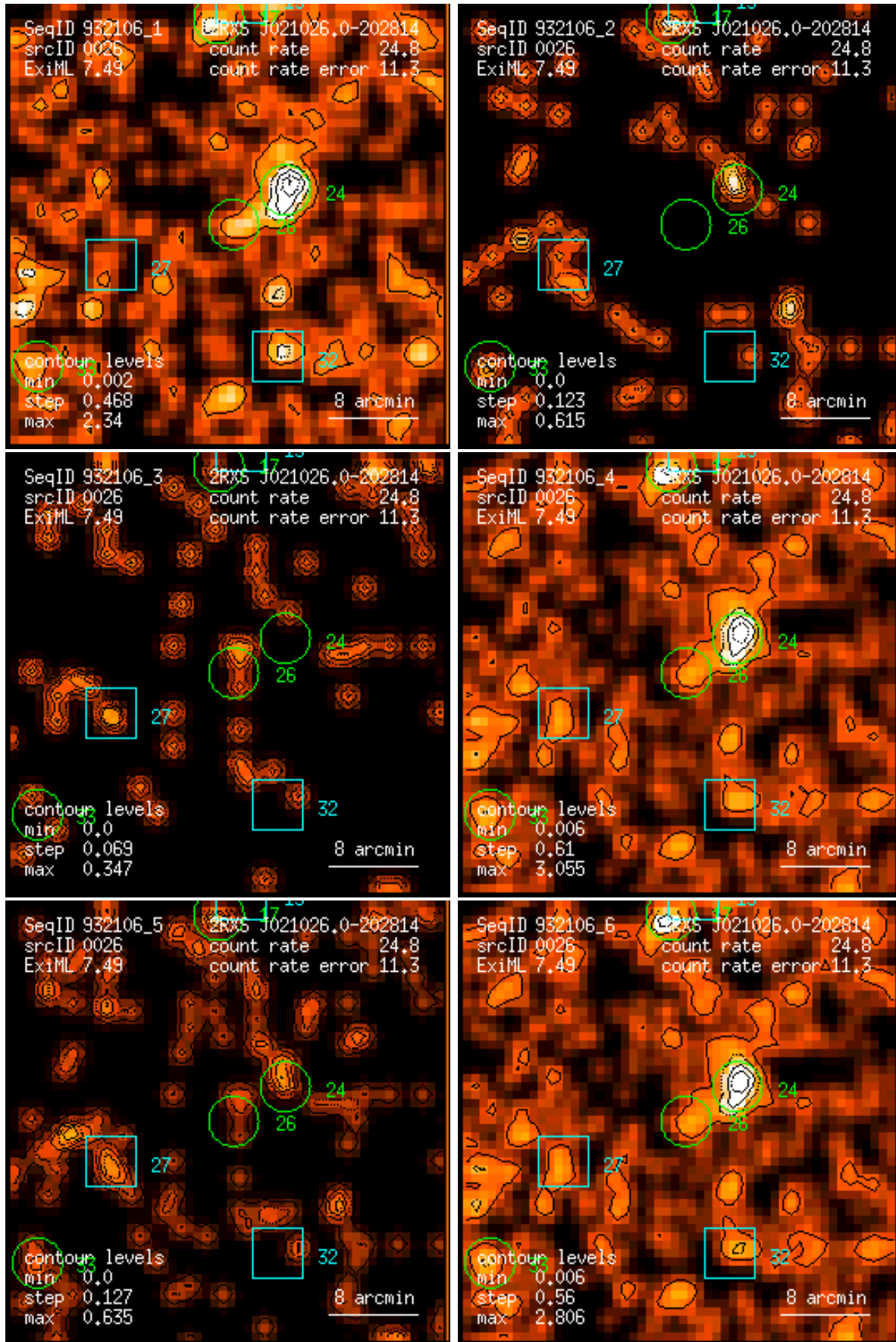
Figure 26: RASS 932106: detection 0026: band rate images, Gaussian filter: (1) PSPC channels 11 – 41, (2) 52 – 90, (3) 91 – 201, (4) 11 – 235, (5) 52 – 201, (6) 11 – 201. Broad band rates in counts/ks. Band rate contour levels in counts/ks/arcmin 2 .
