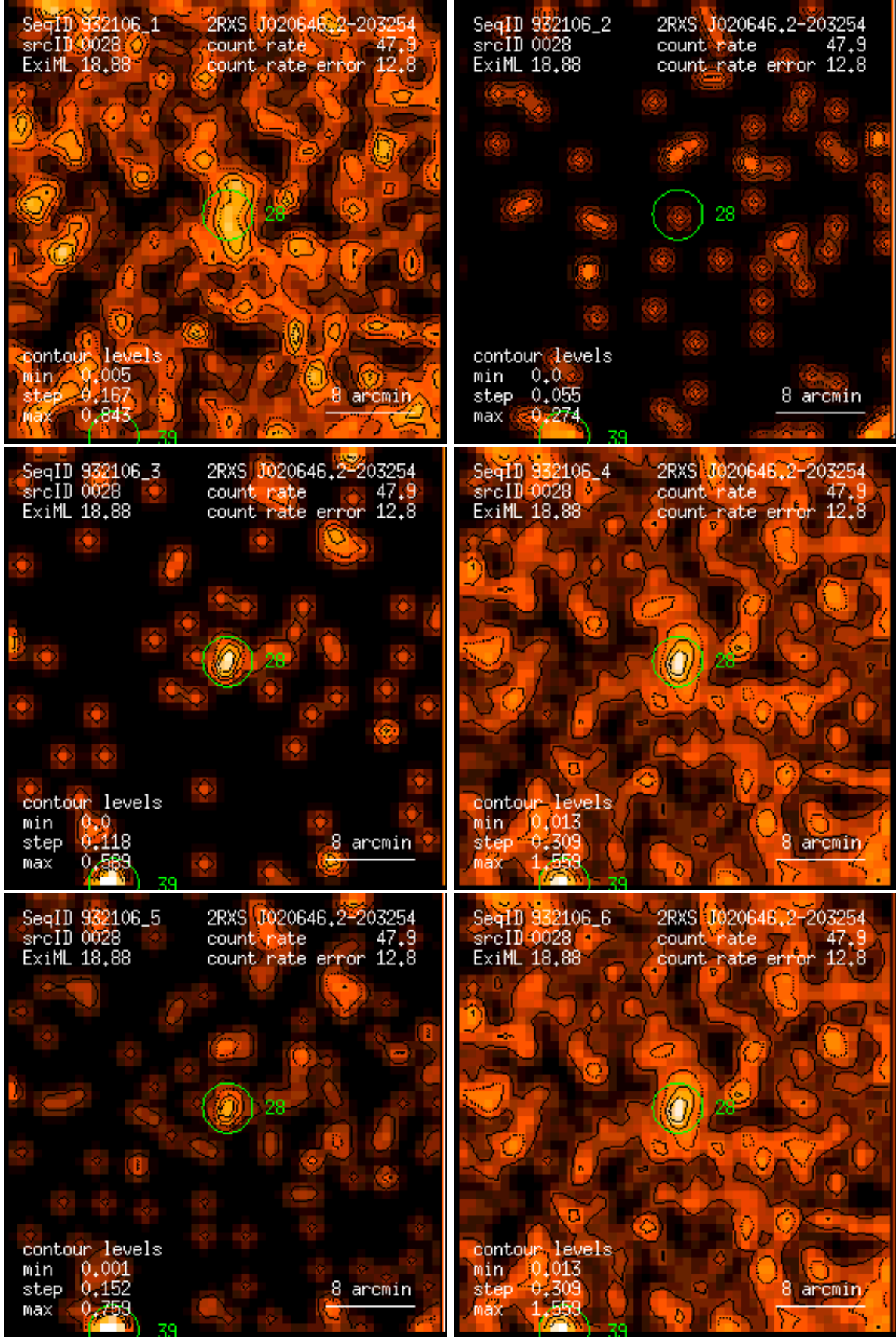
Figure 28: RASS 932106: detection 0028: band rate images, Gaussian filter: (1) PSPC channels 11 – 41, (2) 52 – 90, (3) 91 – 201, (4) 11 – 235, (5) 52 – 201, (6) 11 – 201. Broad band rates in counts/ks. Band rate contour levels in counts/ks/arcmin 2 .
