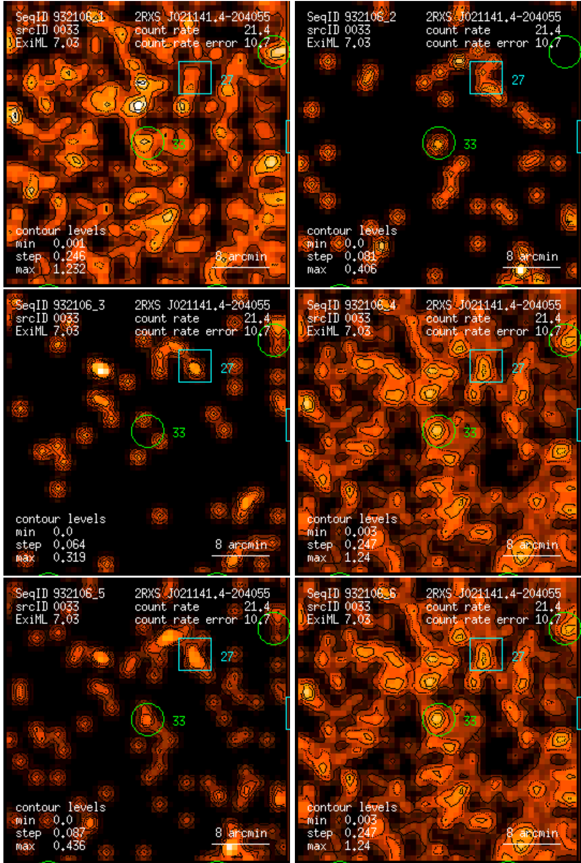
Figure 33: RASS 932106: detection 0033: band rate images, Gaussian filter: (1) PSPC channels 11 – 41, (2) 52 – 90, (3) 91 – 201, (4) 11 – 235, (5) 52 – 201, (6) 11 – 201. Broad band rates in counts/ks. Band rate contour levels in counts/ks/arcmin 2 .
