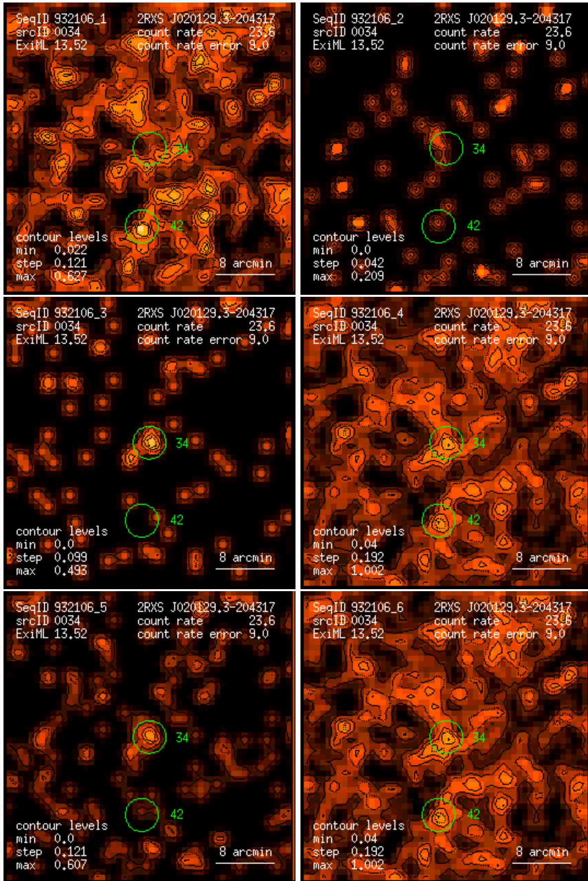
Figure 34: RASS 932106: detection 0034: band rate images, Gaussian filter: (1) PSPC channels 11 – 41, (2) 52 – 90, (3) 91 – 201, (4) 11 – 235, (5) 52 – 201, (6) 11 – 201. Broad band rates in counts/ks. Band rate contour levels in counts/ks/arcmin 2 .
