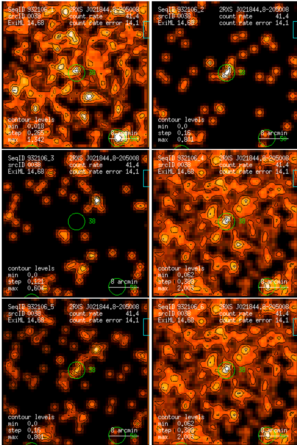
Figure 38: RASS 932106: detection 0038: band rate images, Gaussian filter: (1) PSPC channels 11 – 41, (2) 52 – 90, (3) 91 – 201, (4) 11 – 235, (5) 52 – 201, (6) 11 – 201. Broad band rates in counts/ks. Band rate contour levels in counts/ks/arcmin 2 .
