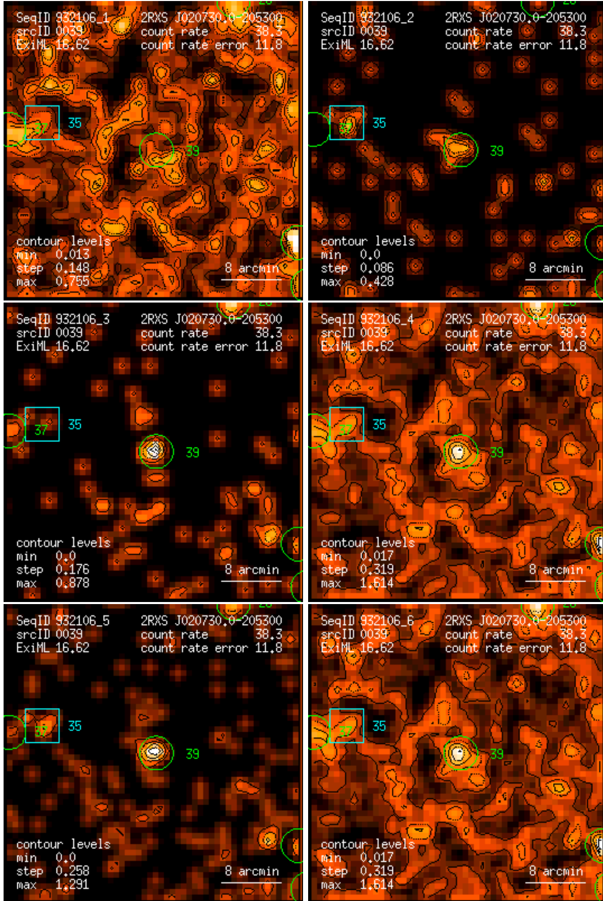
Figure 39: RASS 932106: detection 0039: band rate images, Gaussian filter: (1) PSPC channels 11 – 41, (2) 52 – 90, (3) 91 – 201, (4) 11 – 235, (5) 52 – 201, (6) 11 – 201. Broad band rates in counts/ks. Band rate contour levels in counts/ks/arcmin 2 .
