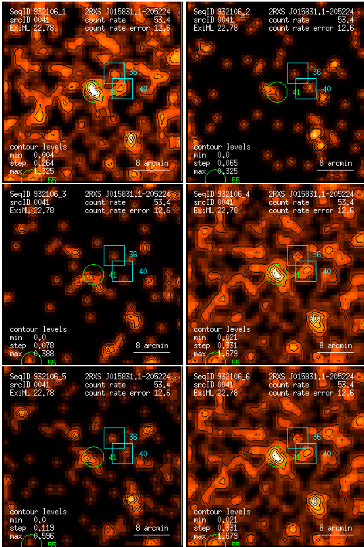
Figure 41: RASS 932106: detection 0041: band rate images, Gaussian filter: (1) PSPC channels 11 – 41, (2) 52 – 90, (3) 91 – 201, (4) 11 – 235, (5) 52 – 201, (6) 11 – 201. Broad band rates in counts/ks. Band rate contour levels in counts/ks/arcmin 2 .
