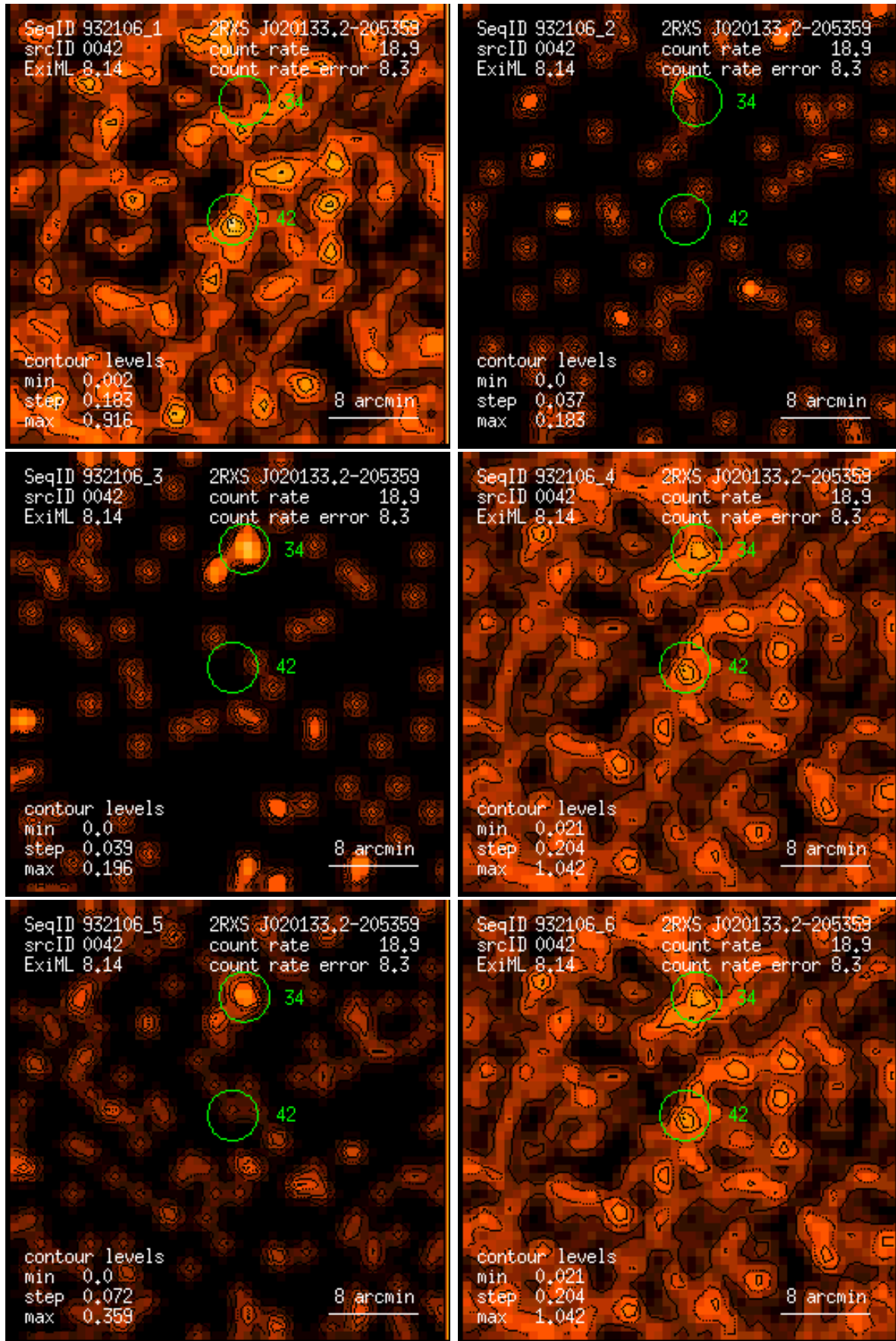
Figure 42: RASS 932106: detection 0042: band rate images, Gaussian filter: (1) PSPC channels 11 – 41, (2) 52 – 90, (3) 91 – 201, (4) 11 – 235, (5) 52 – 201, (6) 11 – 201. Broad band rates in counts/ks. Band rate contour levels in counts/ks/arcmin 2 .
