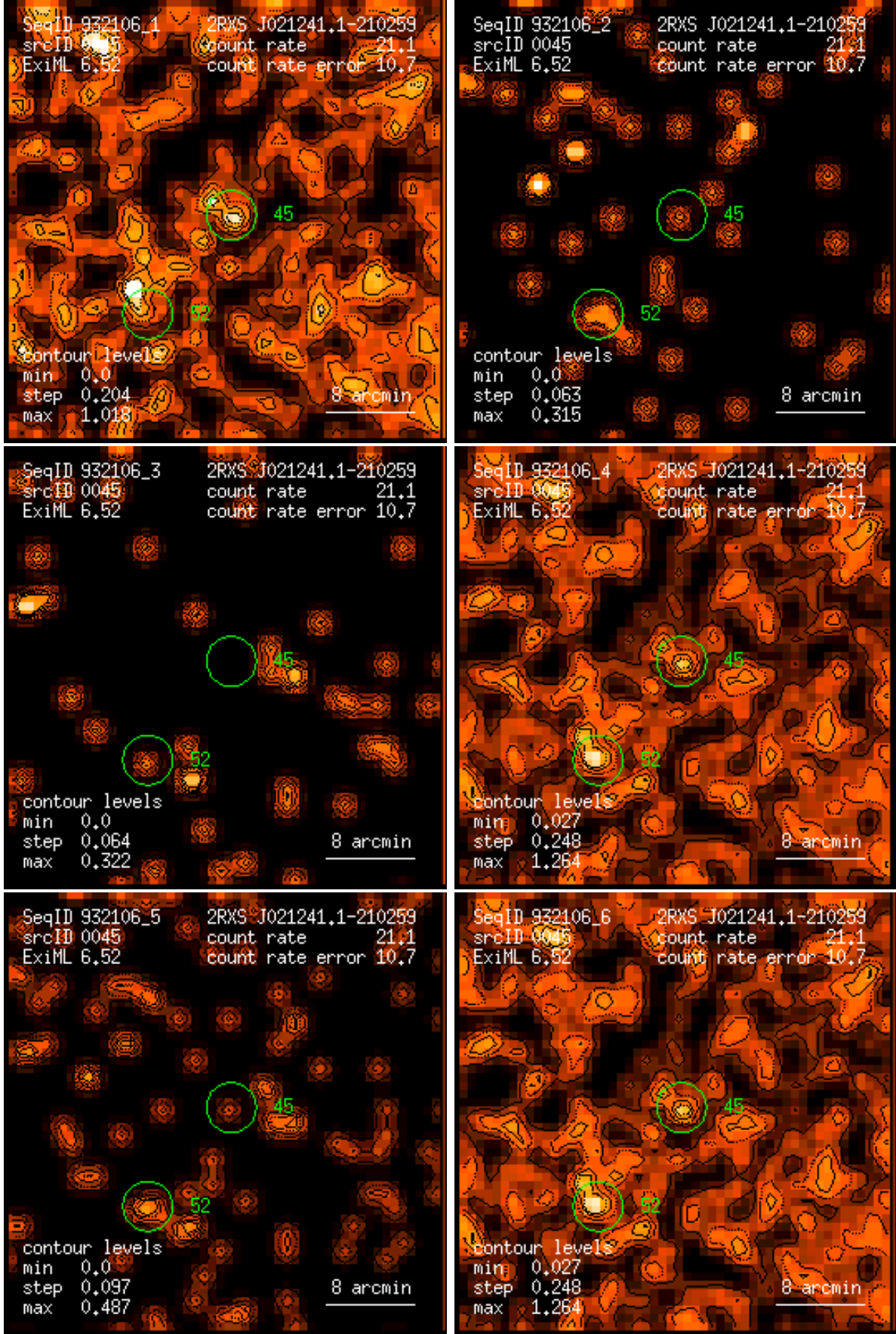
Figure 45: RASS 932106: detection 0045: band rate images, Gaussian filter: (1) PSPC channels 11 – 41, (2) 52 – 90, (3) 91 – 201, (4) 11 – 235, (5) 52 – 201, (6) 11 – 201. Broad band rates in counts/ks. Band rate contour levels in counts/ks/arcmin 2 .
