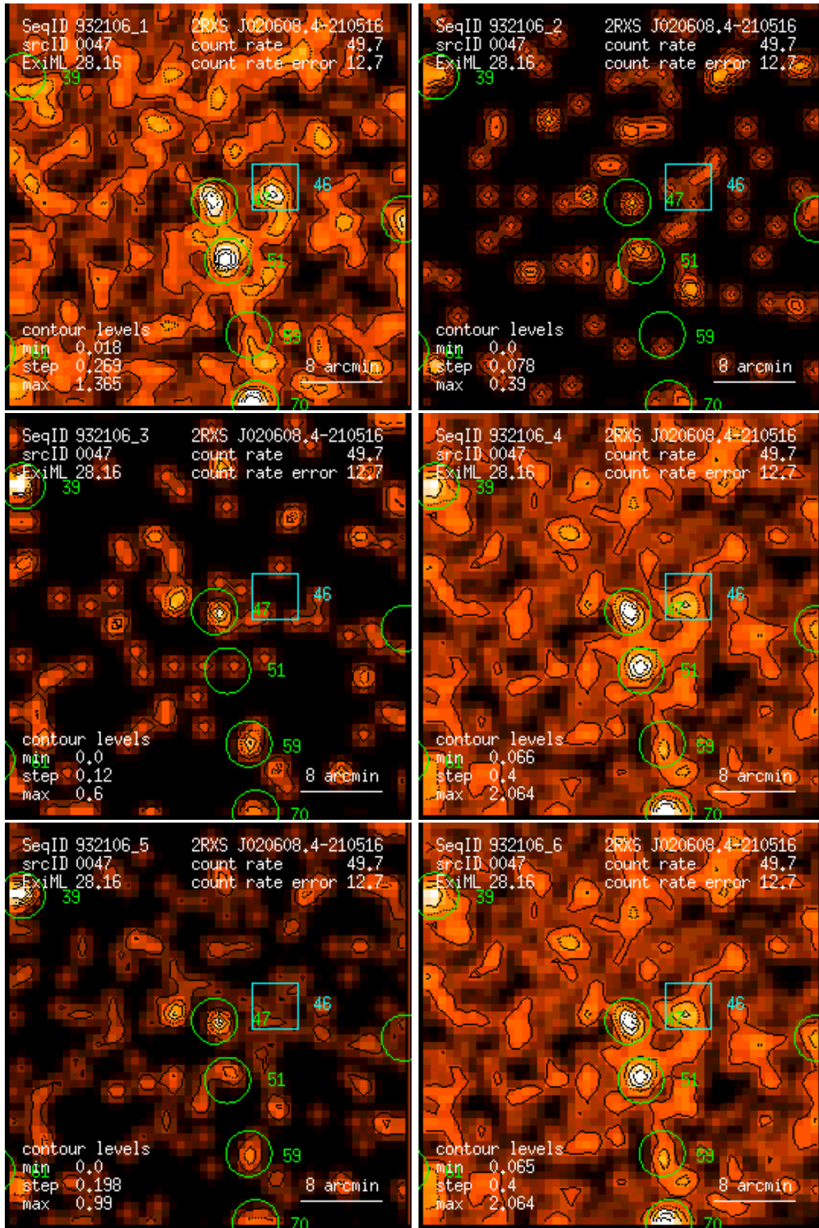
Figure 47: RASS 932106: detection 0047: band rate images, Gaussian filter: (1) PSPC channels 11 – 41, (2) 52 – 90, (3) 91 – 201, (4) 11 – 235, (5) 52 – 201, (6) 11 – 201. Broad band rates in counts/ks. Band rate contour levels in counts/ks/arcmin 2 .
