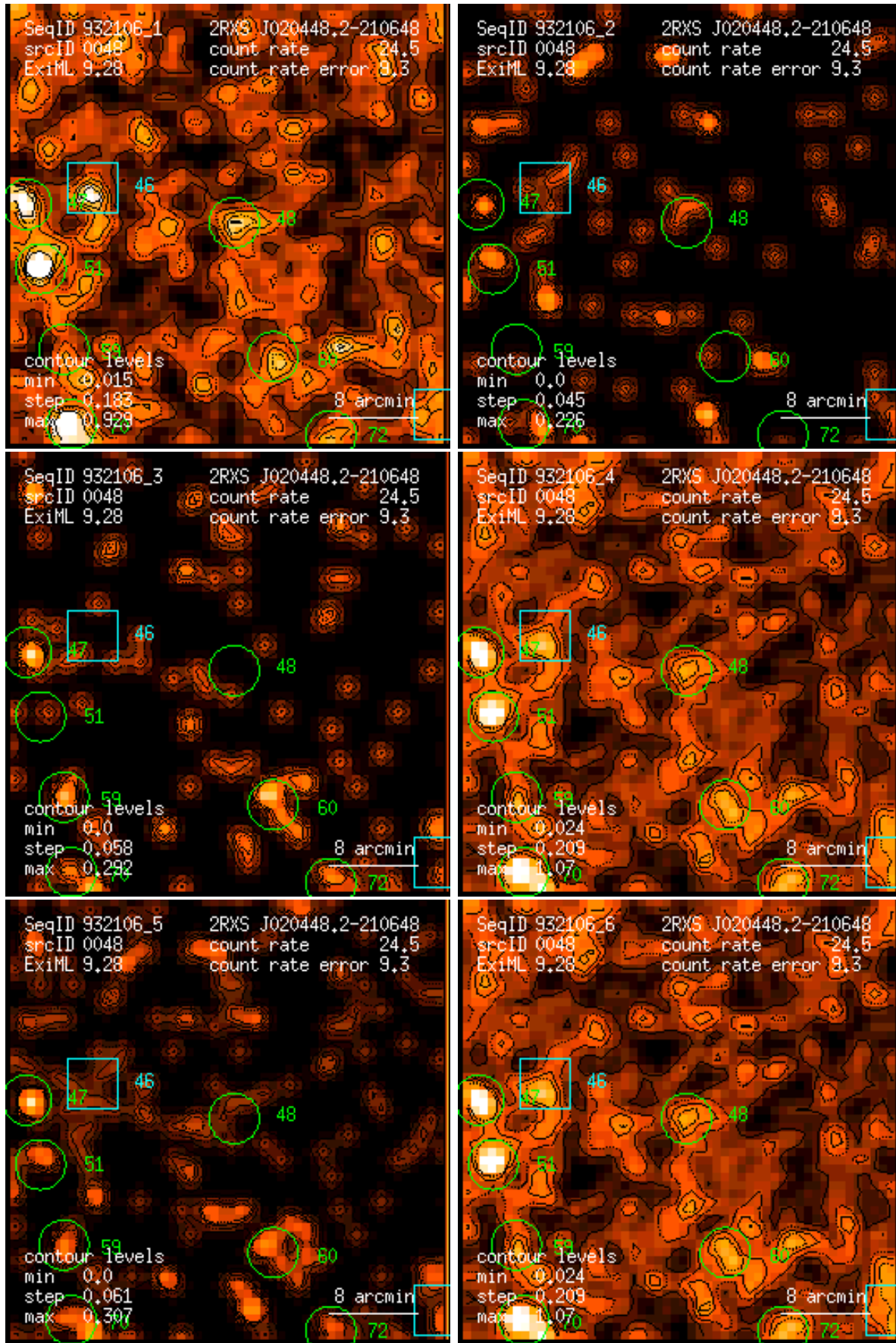
Figure 48: RASS 932106: detection 0048: band rate images, Gaussian filter: (1) PSPC channels 11 – 41, (2) 52 – 90, (3) 91 – 201, (4) 11 – 235, (5) 52 – 201, (6) 11 – 201. Broad band rates in counts/ks. Band rate contour levels in counts/ks/arcmin 2 .
