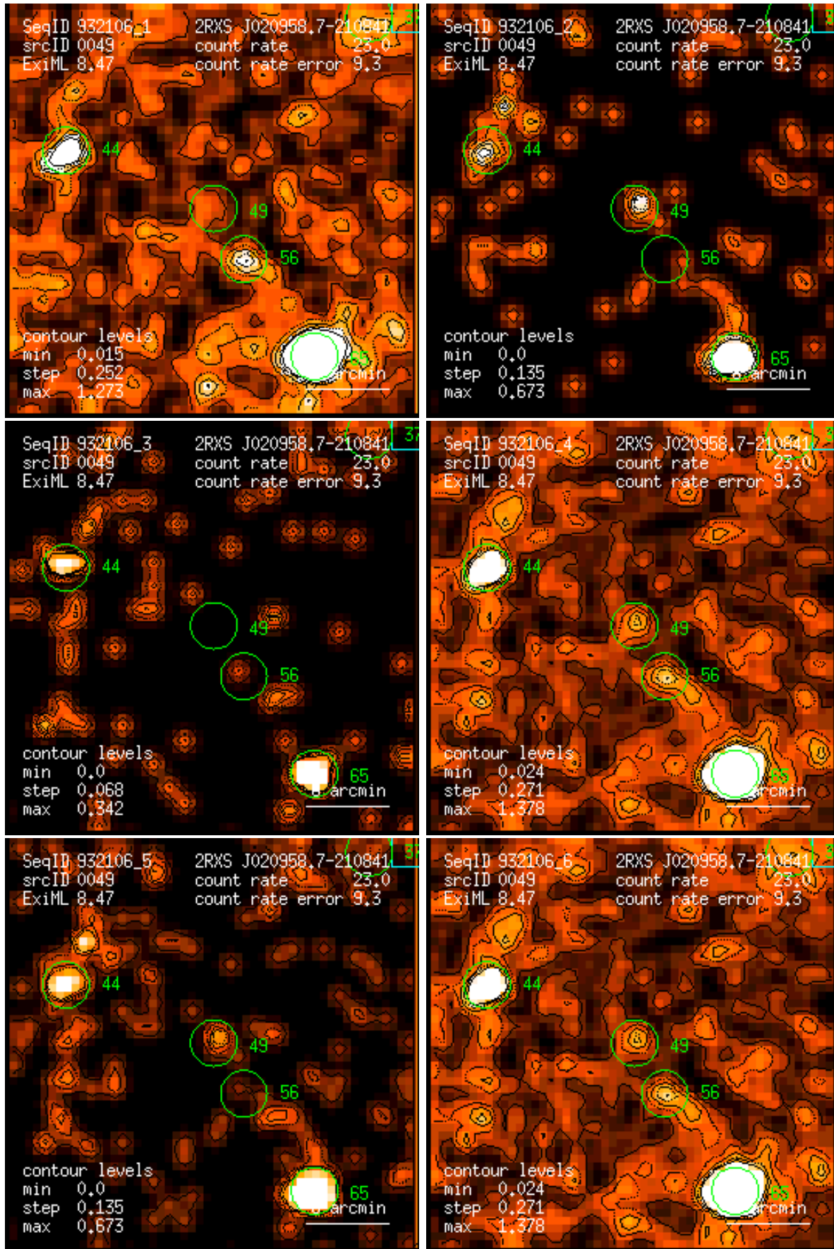
Figure 49: RASS 932106: detection 0049: band rate images, Gaussian filter: (1) PSPC channels 11 – 41, (2) 52 – 90, (3) 91 – 201, (4) 11 – 235, (5) 52 – 201, (6) 11 – 201. Broad band rates in counts/ks. Band rate contour levels in counts/ks/arcmin 2 .
