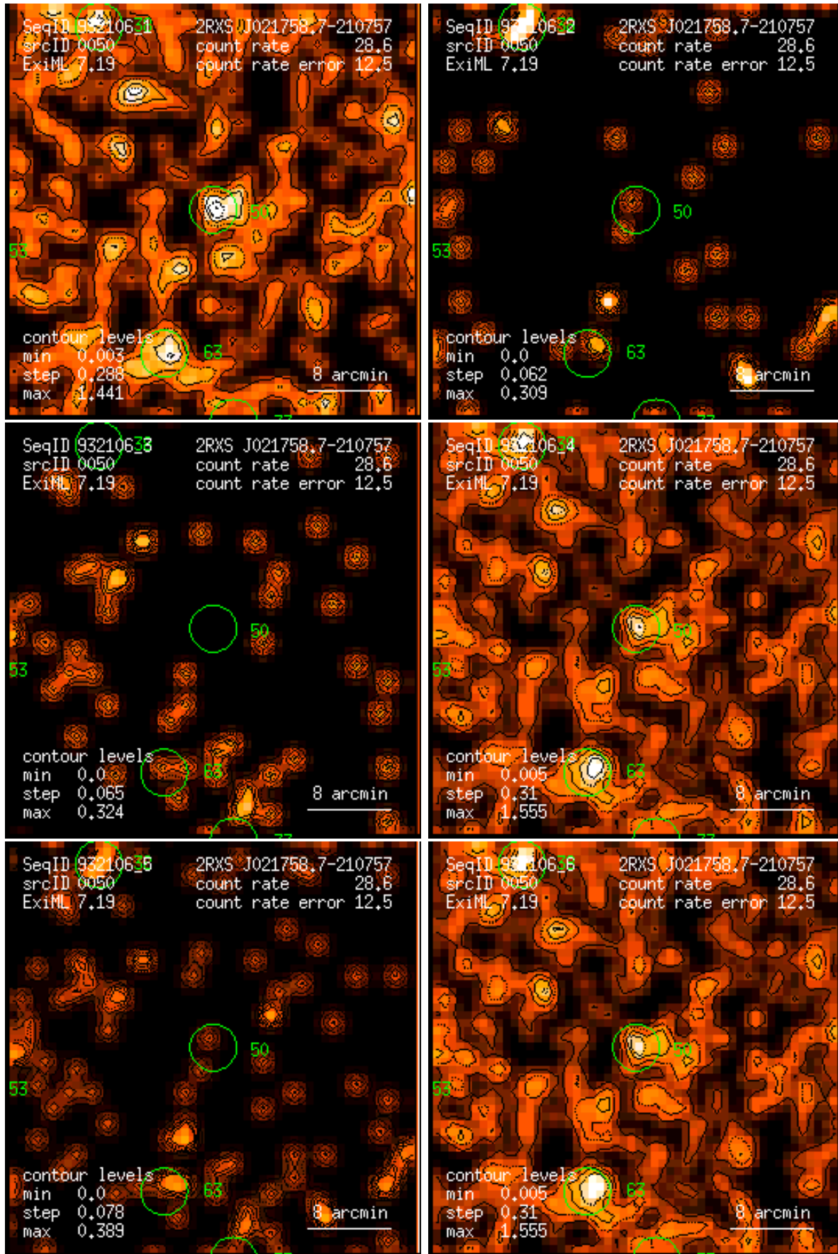
Figure 50: RASS 932106: detection 0050: band rate images, Gaussian filter: (1) PSPC channels 11 – 41, (2) 52 – 90, (3) 91 – 201, (4) 11 – 235, (5) 52 – 201, (6) 11 – 201. Broad band rates in counts/ks. Band rate contour levels in counts/ks/arcmin 2 .
