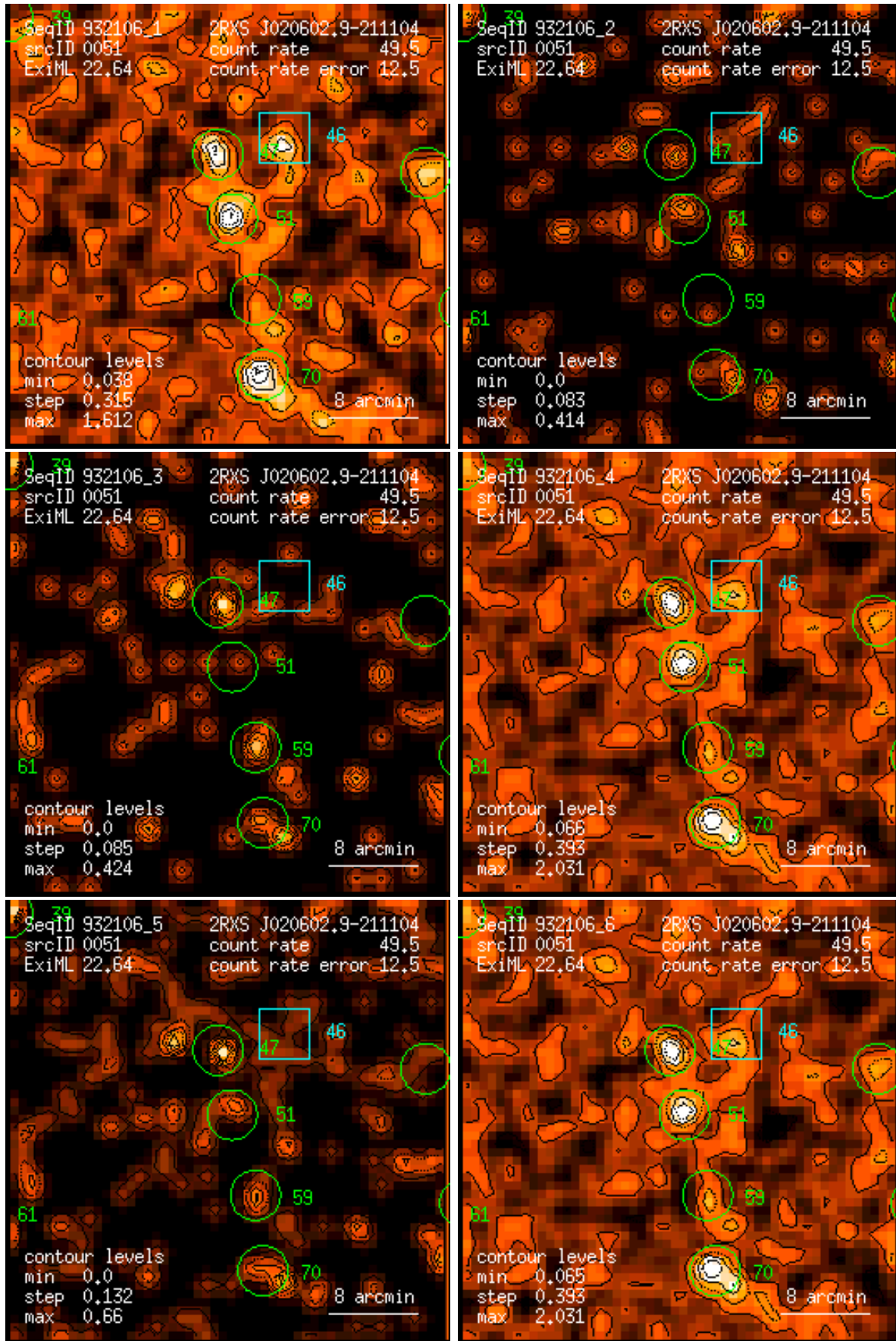
Figure 51: RASS 932106: detection 0051: band rate images, Gaussian filter: (1) PSPC channels 11 – 41, (2) 52 – 90, (3) 91 – 201, (4) 11 – 235, (5) 52 – 201, (6) 11 – 201. Broad band rates in counts/ks. Band rate contour levels in counts/ks/arcmin 2 .
