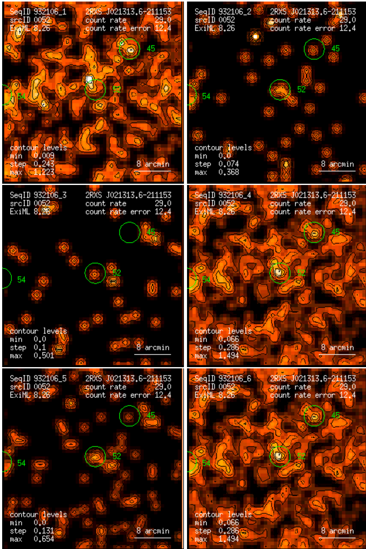
Figure 52: RASS 932106: detection 0052: band rate images, Gaussian filter: (1) PSPC channels 11 – 41, (2) 52 – 90, (3) 91 – 201, (4) 11 – 235, (5) 52 – 201, (6) 11 – 201. Broad band rates in counts/ks. Band rate contour levels in counts/ks/arcmin 2 .
