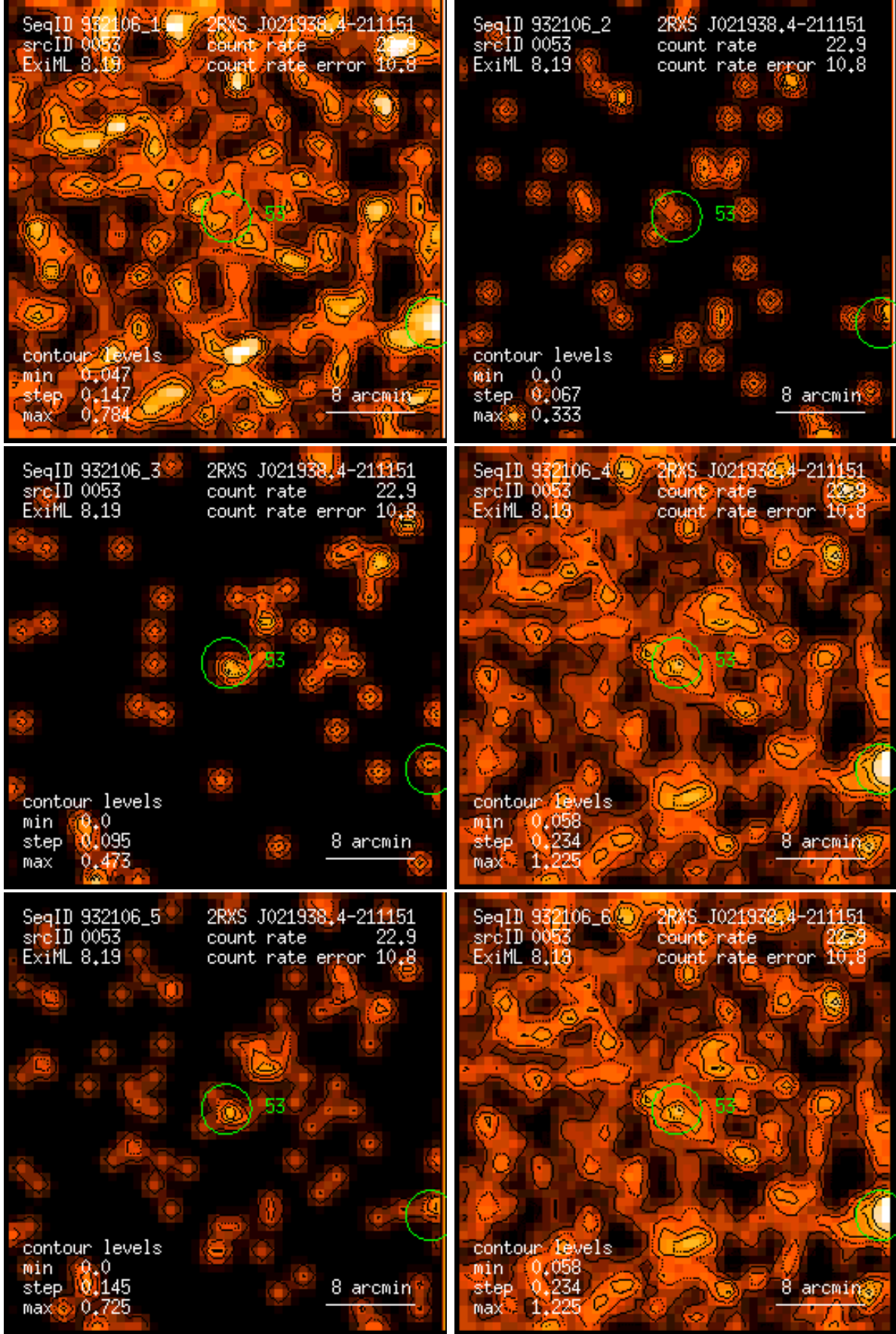
Figure 53: RASS 932106: detection 0053: band rate images, Gaussian filter: (1) PSPC channels 11 – 41, (2) 52 – 90, (3) 91 – 201, (4) 11 – 235, (5) 52 – 201, (6) 11 – 201. Broad band rates in counts/ks. Band rate contour levels in counts/ks/arcmin 2 .
