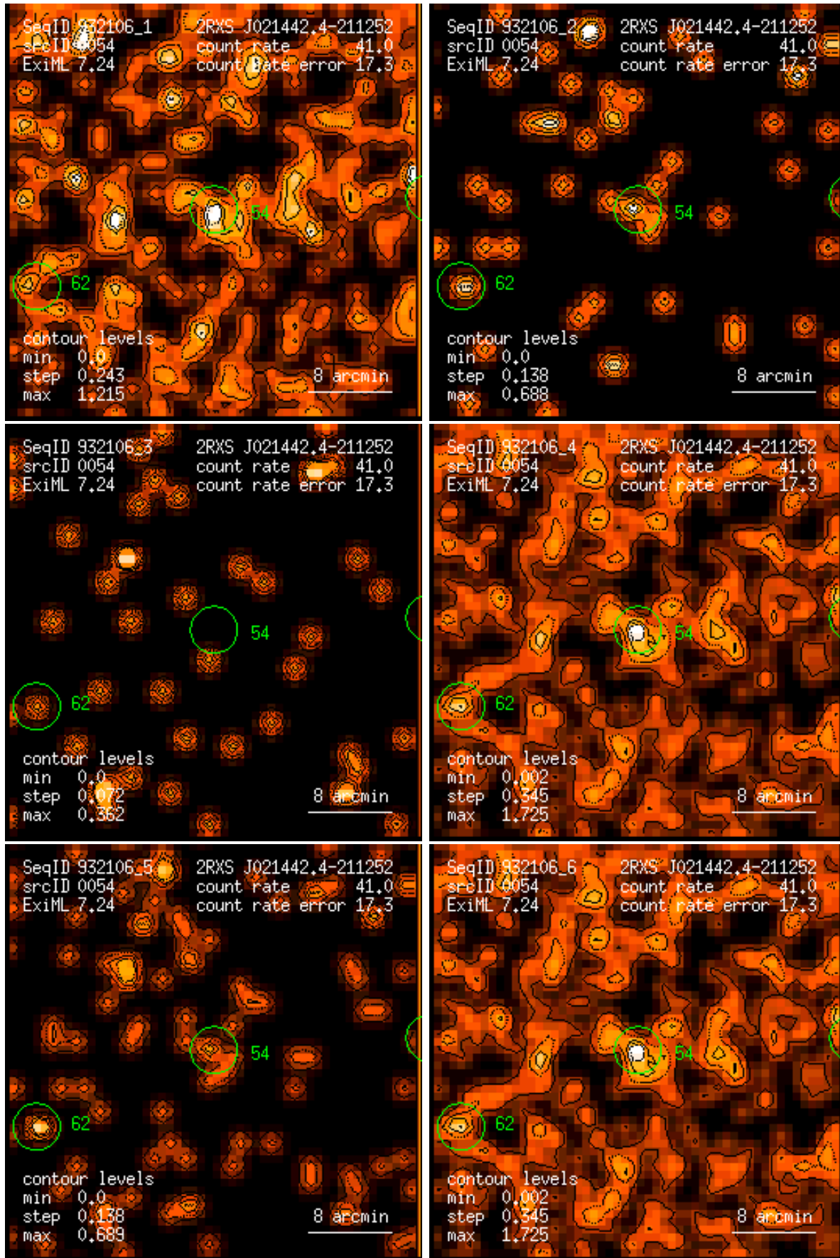
Figure 54: RASS 932106: detection 0054: band rate images, Gaussian filter: (1) PSPC channels 11 – 41, (2) 52 – 90, (3) 91 – 201, (4) 11 – 235, (5) 52 – 201, (6) 11 – 201. Broad band rates in counts/ks. Band rate contour levels in counts/ks/arcmin 2 .
