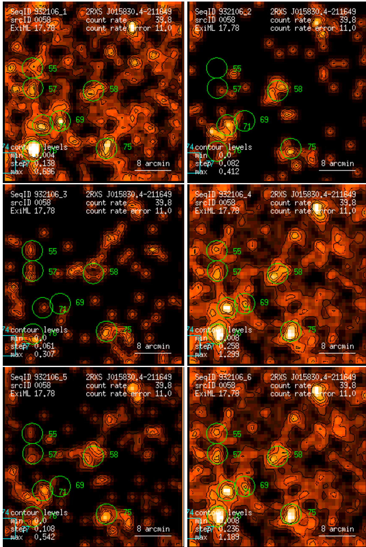
Figure 58: RASS 932106: detection 0058: band rate images, Gaussian filter: (1) PSPC channels 11 – 41, (2) 52 – 90, (3) 91 – 201, (4) 11 – 235, (5) 52 – 201, (6) 11 – 201. Broad band rates in counts/ks. Band rate contour levels in counts/ks/arcmin 2 .
