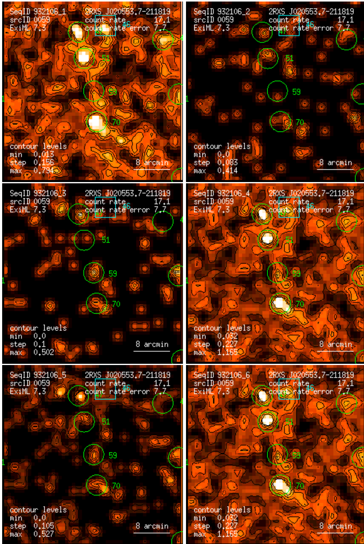
Figure 59: RASS 932106: detection 0059: band rate images, Gaussian filter: (1) PSPC channels 11 – 41, (2) 52 – 90, (3) 91 – 201, (4) 11 – 235, (5) 52 – 201, (6) 11 – 201. Broad band rates in counts/ks. Band rate contour levels in counts/ks/arcmin 2 .
