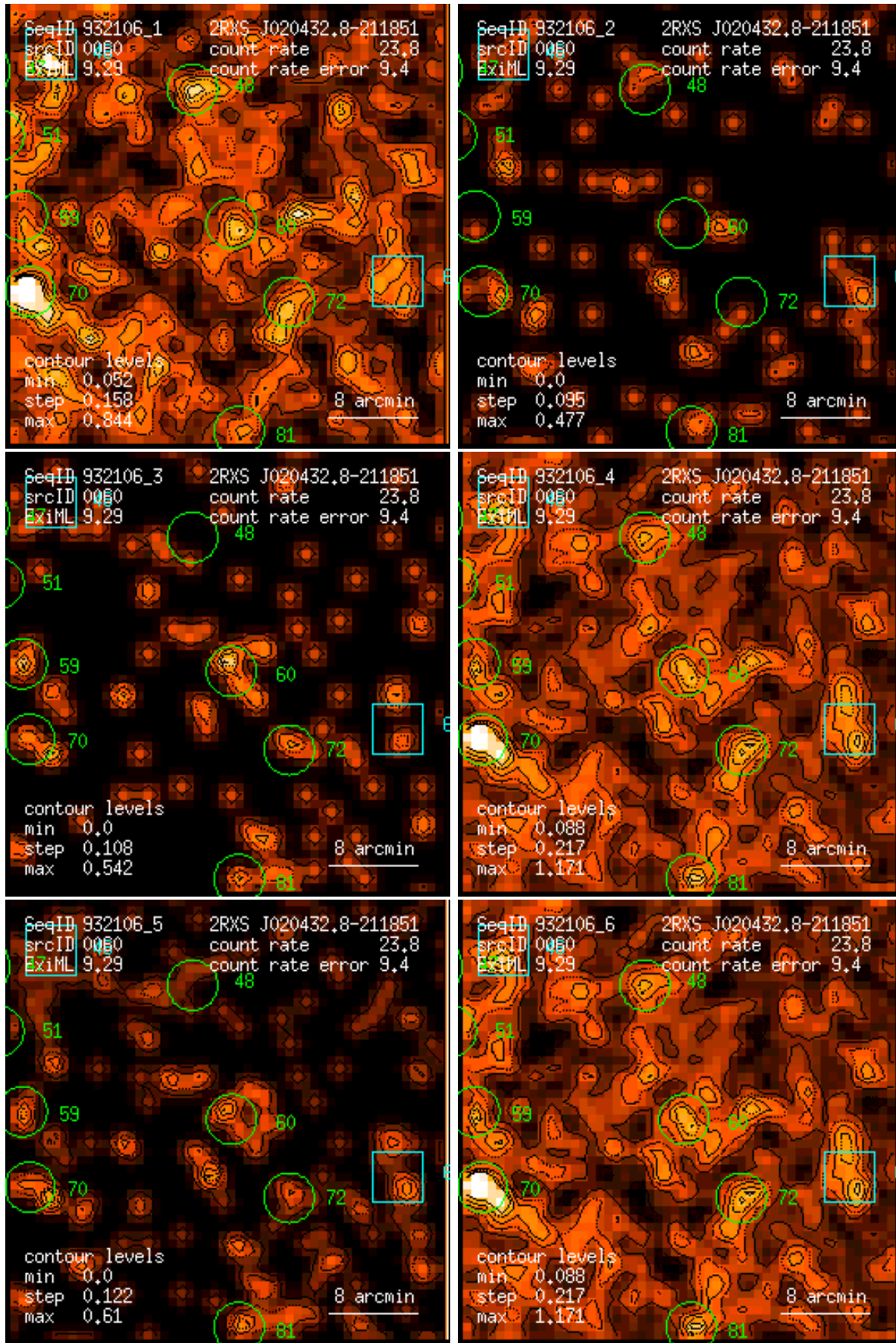
Figure 60: RASS 932106: detection 0060: band rate images, Gaussian filter: (1) PSPC channels 11 – 41, (2) 52 – 90, (3) 91 – 201, (4) 11 – 235, (5) 52 – 201, (6) 11 – 201. Broad band rates in counts/ks. Band rate contour levels in counts/ks/arcmin 2 .
