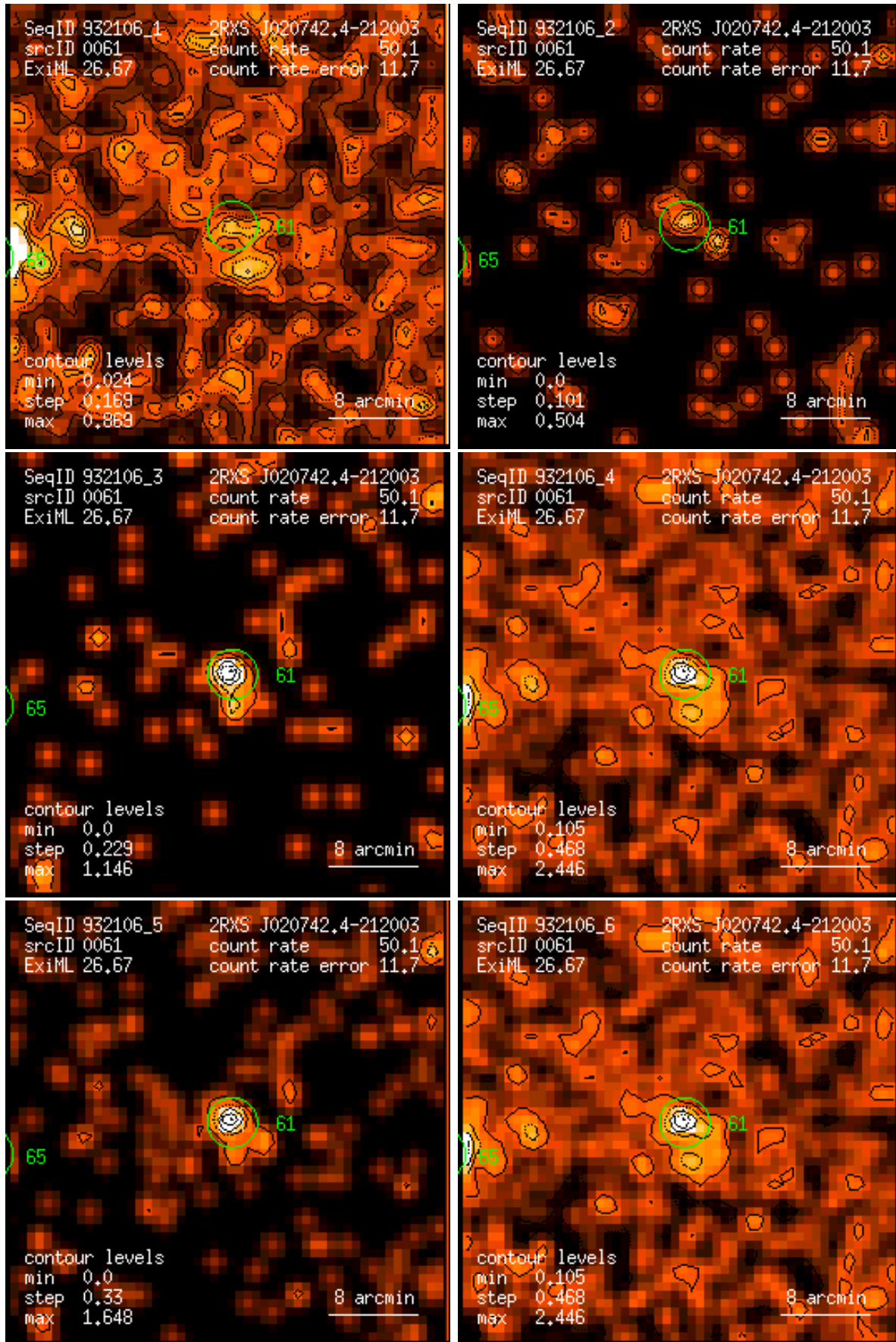
Figure 61: RASS 932106: detection 0061: band rate images, Gaussian filter: (1) PSPC channels 11 – 41, (2) 52 – 90, (3) 91 – 201, (4) 11 – 235, (5) 52 – 201, (6) 11 – 201. Broad band rates in counts/ks. Band rate contour levels in counts/ks/arcmin 2 .
