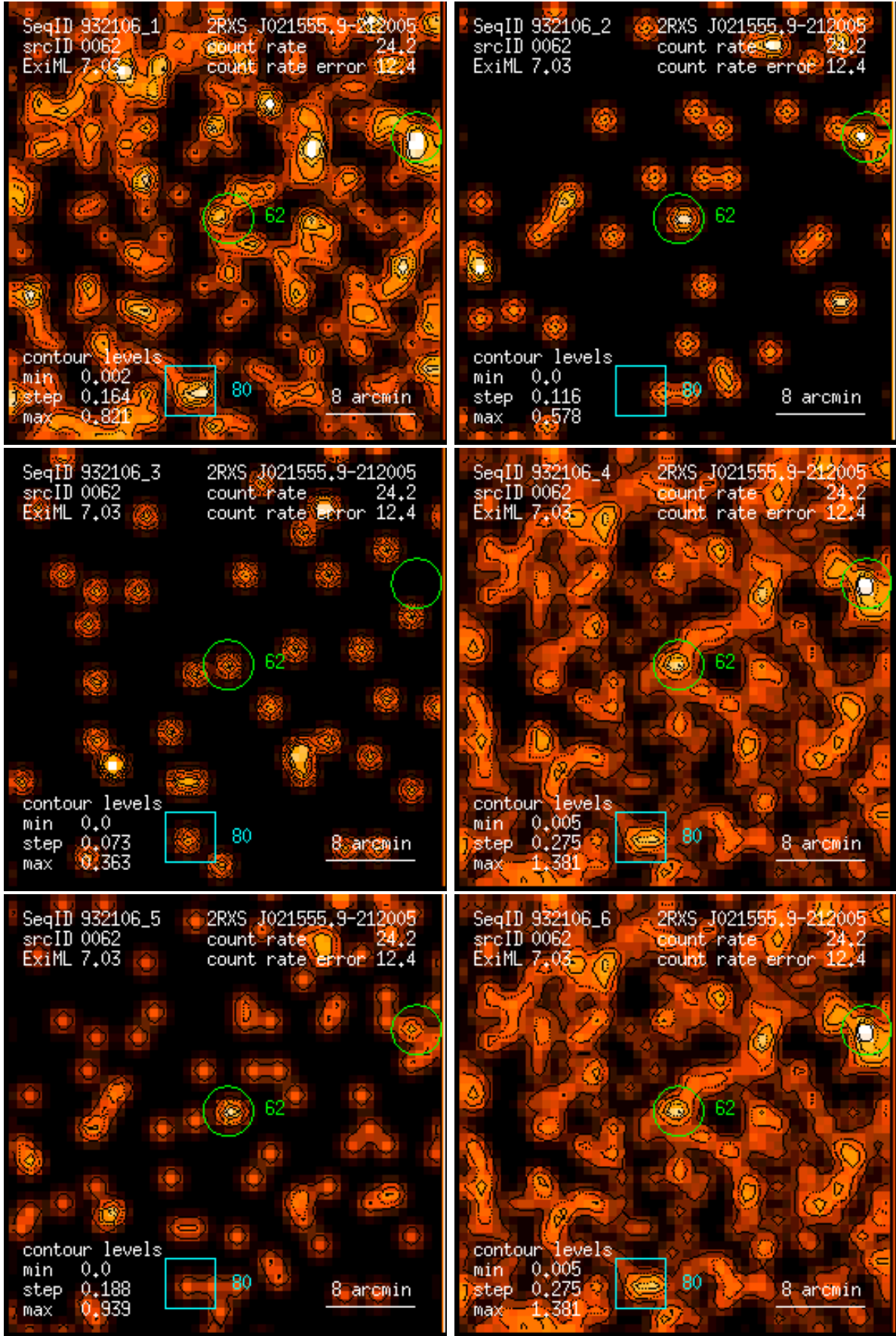
Figure 62: RASS 932106: detection 0062: band rate images, Gaussian filter: (1) PSPC channels 11 – 41, (2) 52 – 90, (3) 91 – 201, (4) 11 – 235, (5) 52 – 201, (6) 11 – 201. Broad band rates in counts/ks. Band rate contour levels in counts/ks/arcmin 2 .
