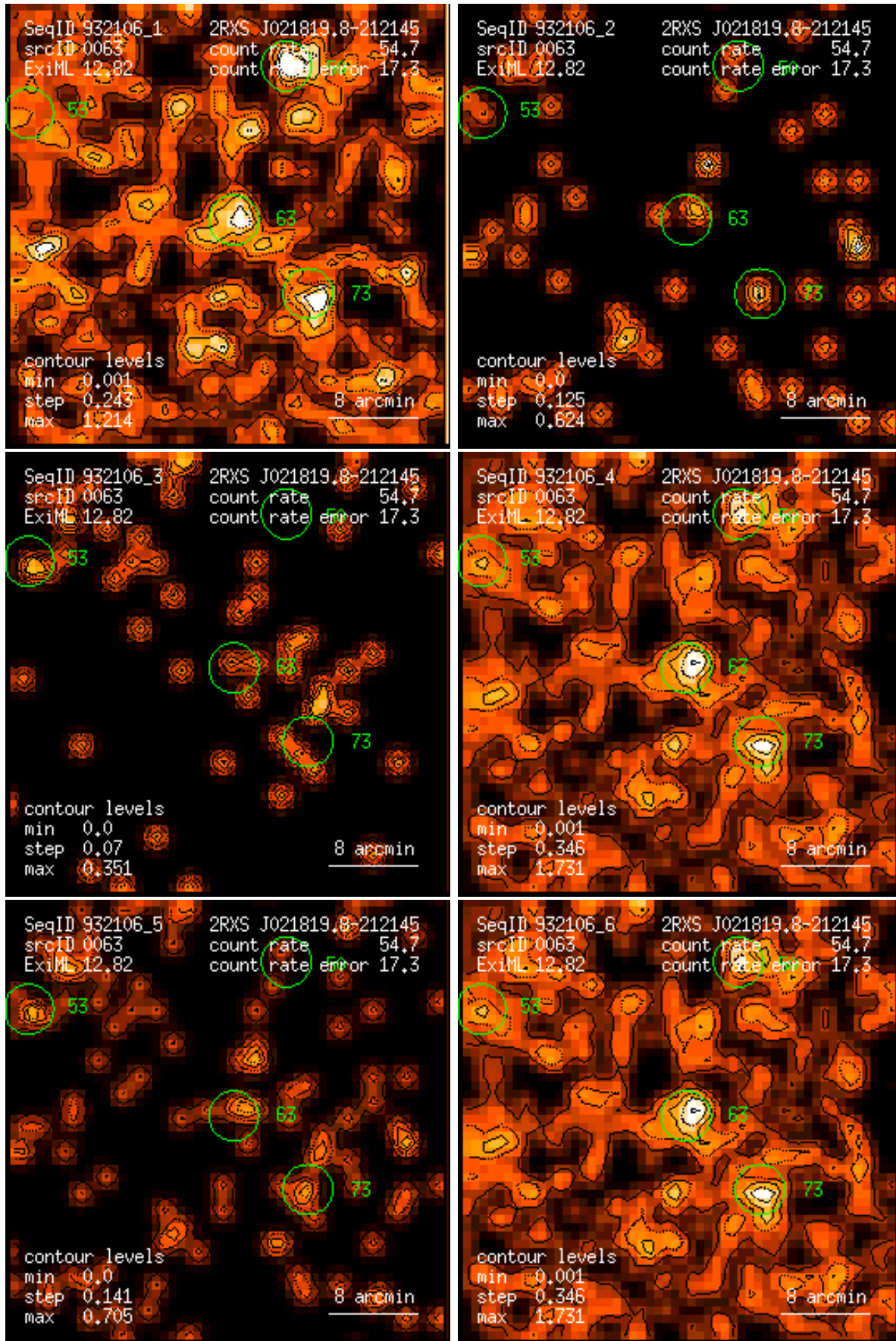
Figure 63: RASS 932106: detection 0063: band rate images, Gaussian filter: (1) PSPC channels 11 – 41, (2) 52 – 90, (3) 91 – 201, (4) 11 – 235, (5) 52 – 201, (6) 11 – 201. Broad band rates in counts/ks. Band rate contour levels in counts/ks/arcmin 2 .
