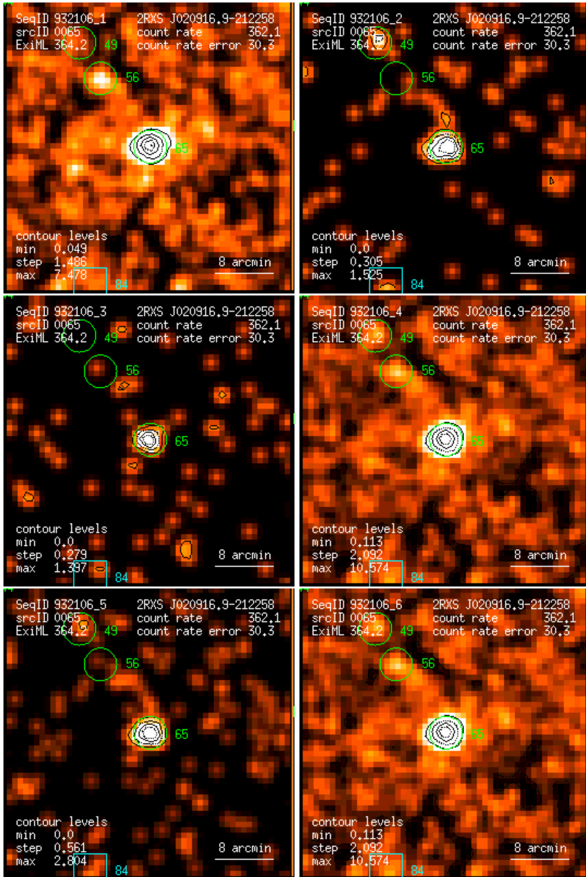
Figure 65: RASS 932106: detection 0065: band rate images, Gaussian filter: (1) PSPC channels 11 – 41, (2) 52 – 90, (3) 91 – 201, (4) 11 – 235, (5) 52 – 201, (6) 11 – 201. Broad band rates in counts/ks. Band rate contour levels in counts/ks/arcmin 2 .
