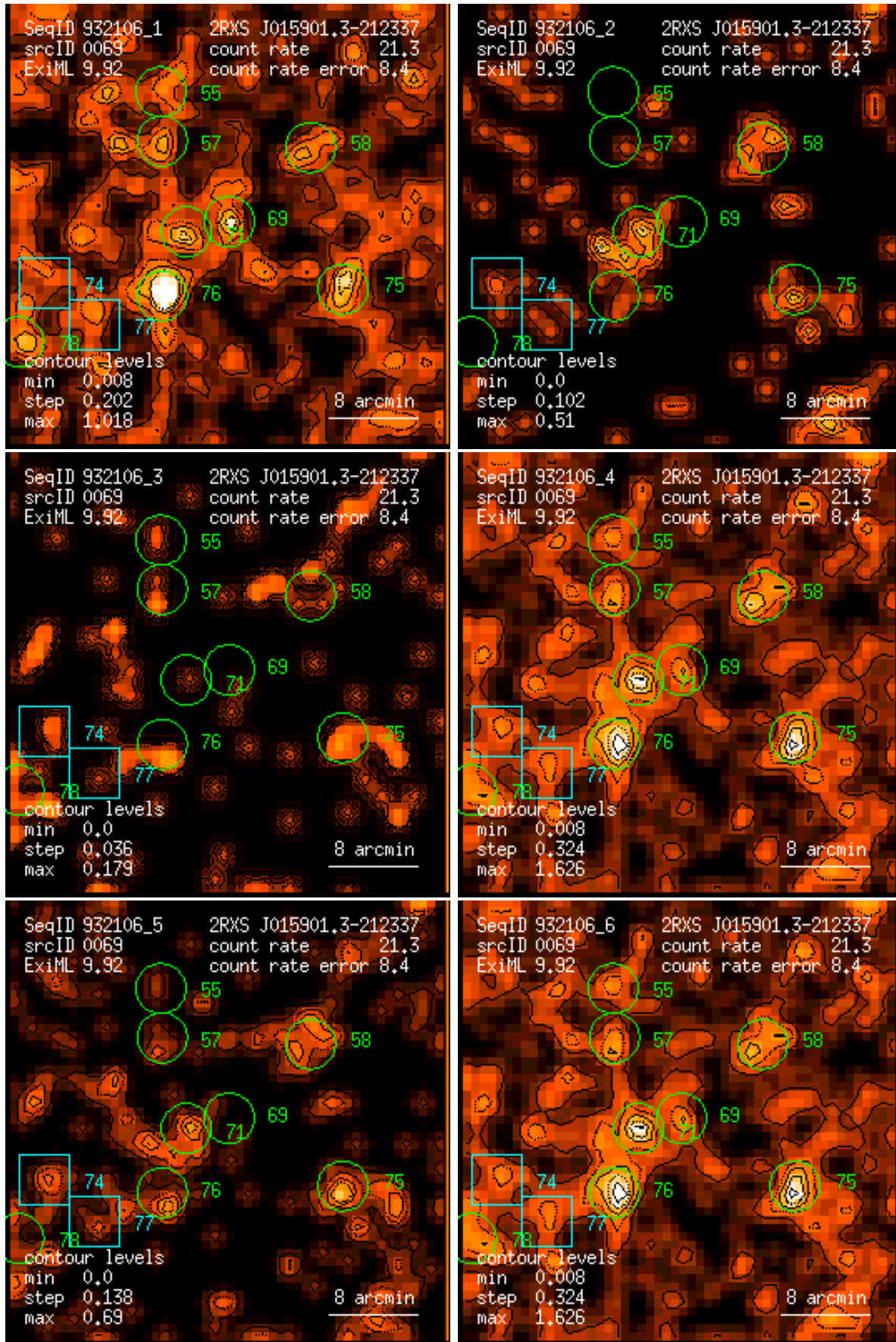
Figure 69: RASS 932106: detection 0069: band rate images, Gaussian filter: (1) PSPC channels 11 – 41, (2) 52 – 90, (3) 91 – 201, (4) 11 – 235, (5) 52 – 201, (6) 11 – 201. Broad band rates in counts/ks. Band rate contour levels in counts/ks/arcmin 2 .
