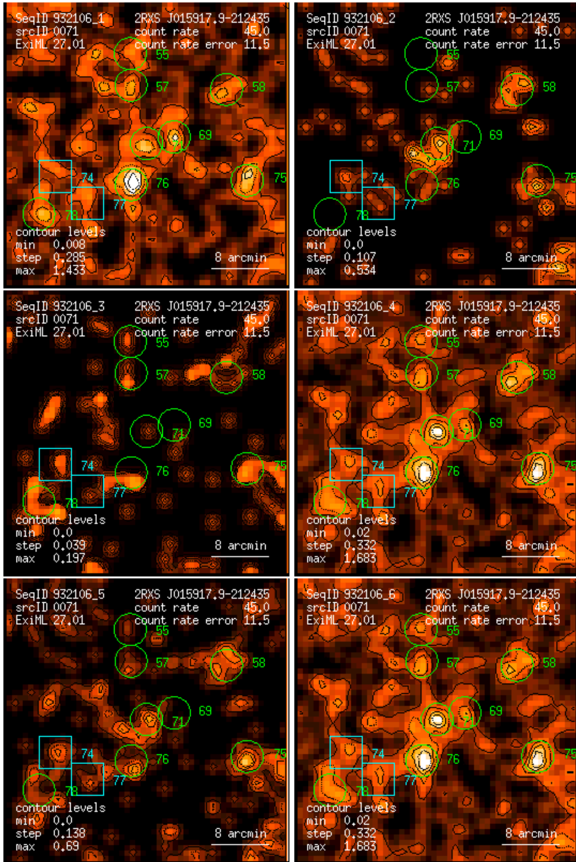
Figure 71: RASS 932106: detection 0071: band rate images, Gaussian filter: (1) PSPC channels 11 – 41, (2) 52 – 90, (3) 91 – 201, (4) 11 – 235, (5) 52 – 201, (6) 11 – 201. Broad band rates in counts/ks. Band rate contour levels in counts/ks/arcmin 2 .
