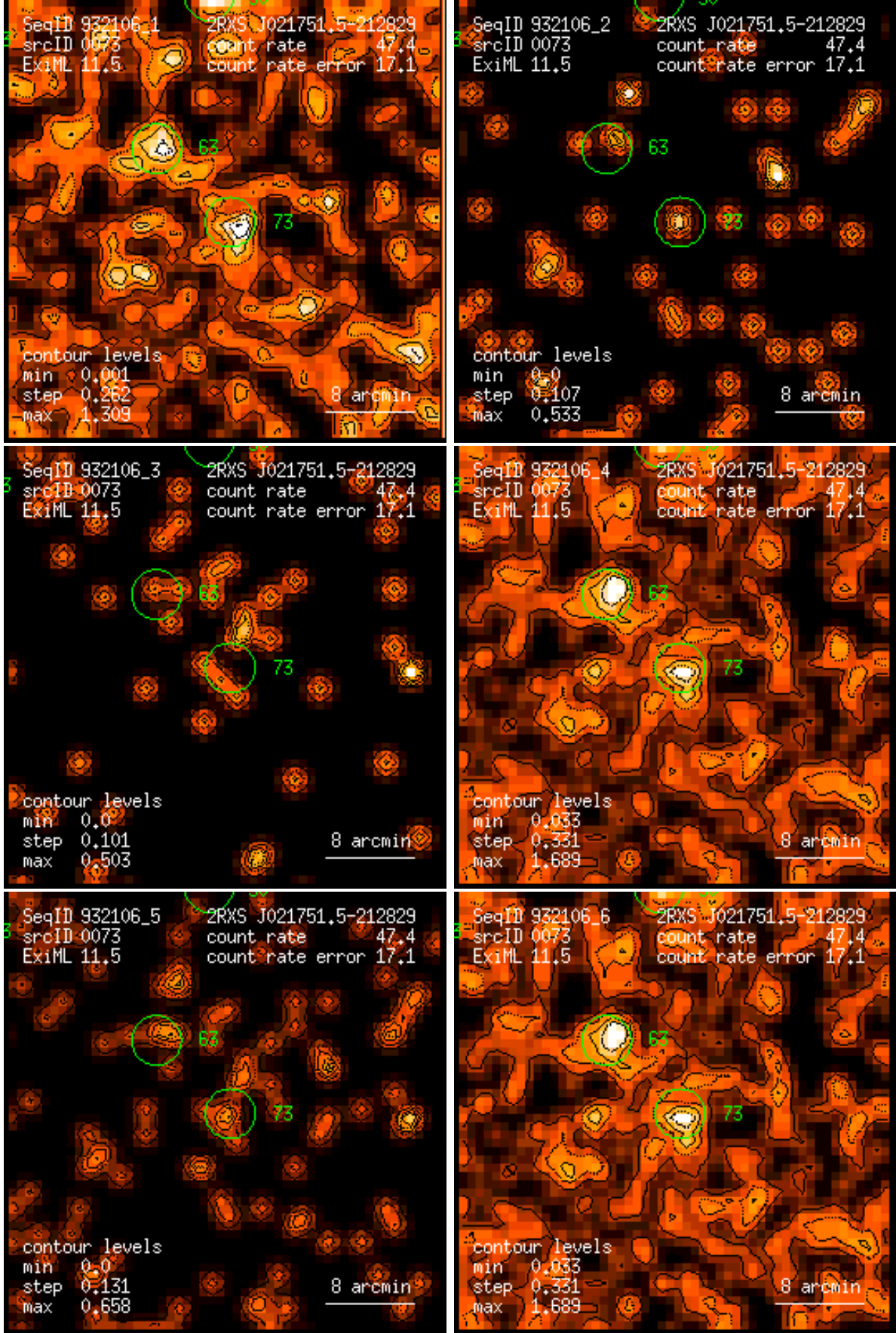
Figure 73: RASS 932106: detection 0073: band rate images, Gaussian filter: (1) PSPC channels 11 – 41, (2) 52 – 90, (3) 91 – 201, (4) 11 – 235, (5) 52 – 201, (6) 11 – 201. Broad band rates in counts/ks. Band rate contour levels in counts/ks/arcmin 2 .
