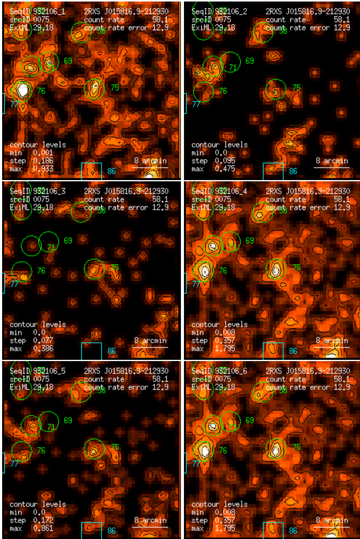
Figure 75: RASS 932106: detection 0075: band rate images, Gaussian filter: (1) PSPC channels 11 – 41, (2) 52 – 90, (3) 91 – 201, (4) 11 – 235, (5) 52 – 201, (6) 11 – 201. Broad band rates in counts/ks. Band rate contour levels in counts/ks/arcmin 2 .
